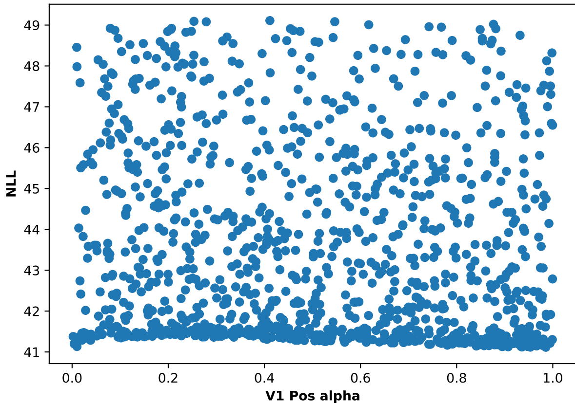
Participant 56, run 2: NLL and V1 Pos alpha scatter plot
