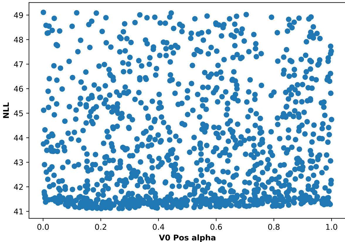
Participant 56, run 2: NLL and V0 Pos alpha scatter plot
