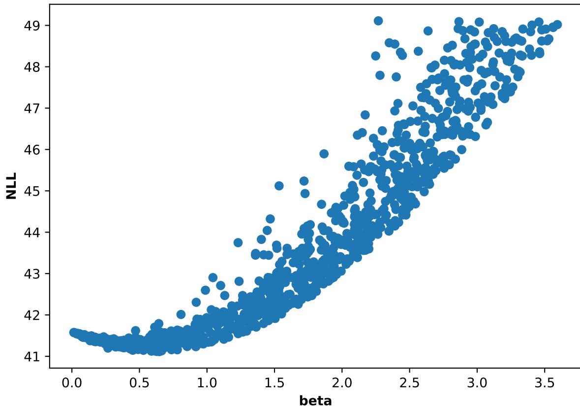
Participant 56, run 2: NLL and beta scatter plot
