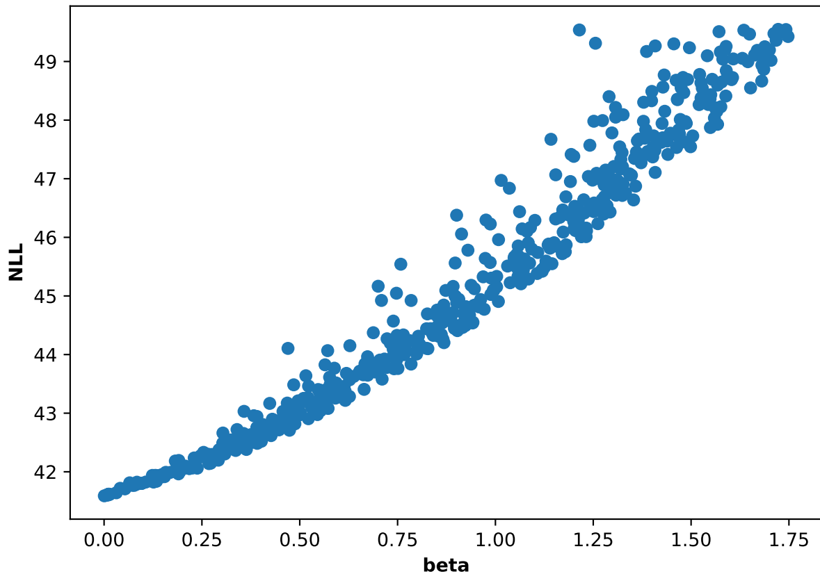
Participant 57, run 1: NLL and beta scatter plot
