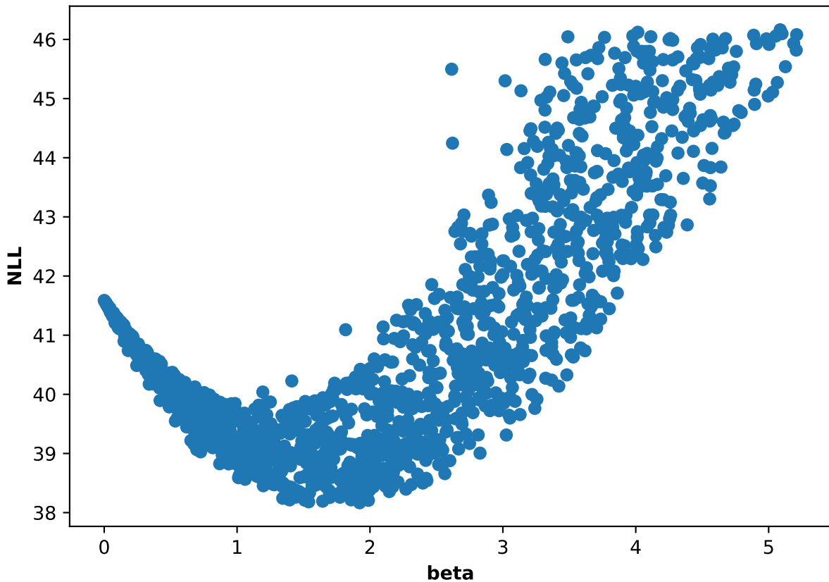
Participant 57, run 2: NLL and beta scatter plot
