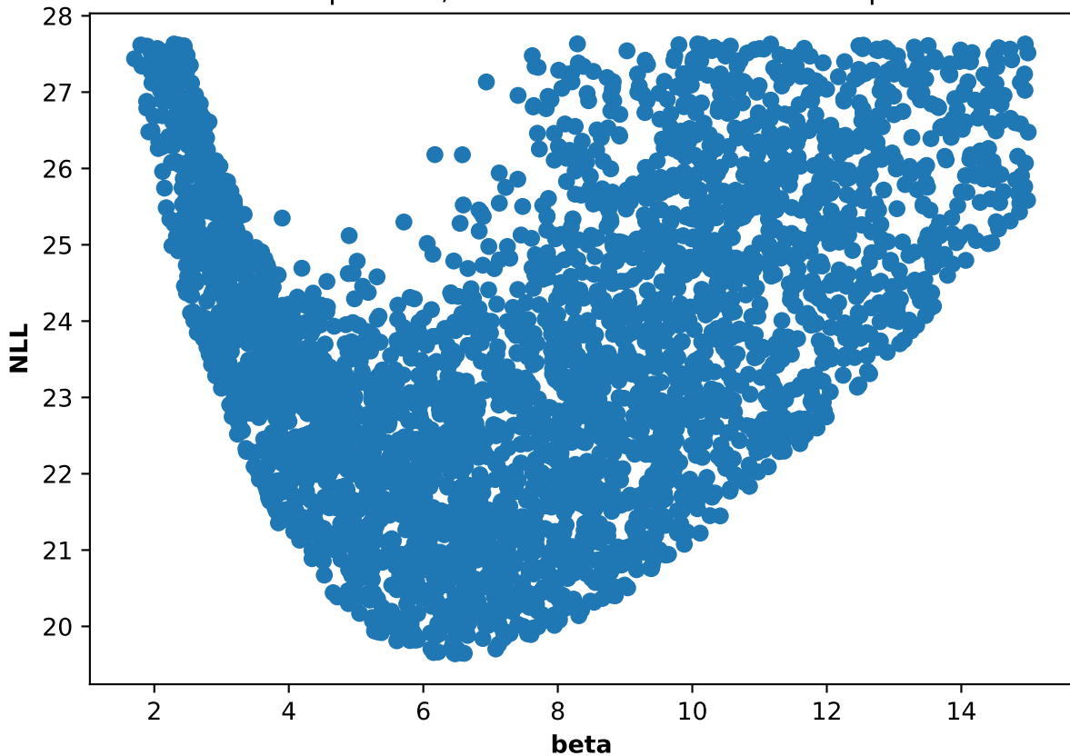
Participant 57, run 5: NLL and beta scatter plot
