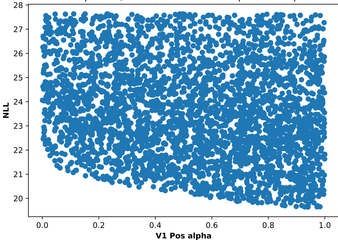
Participant 57, run 5: NLL and V1 Pos alpha scatter plot
