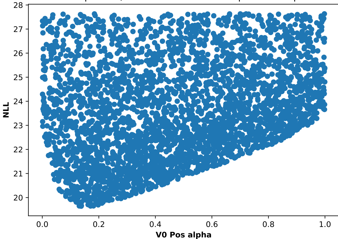
Participant 57, run 5: NLL and V0 Pos alpha scatter plot
