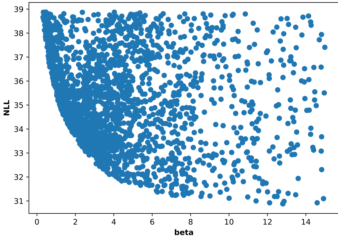
Participant 58, run 2: NLL and beta scatter plot
