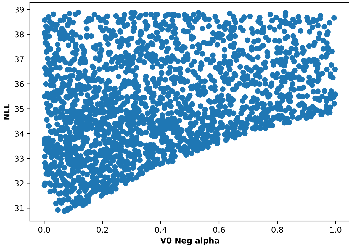
Participant 58, run 2: NLL and V0 Neg alpha scatter plot
