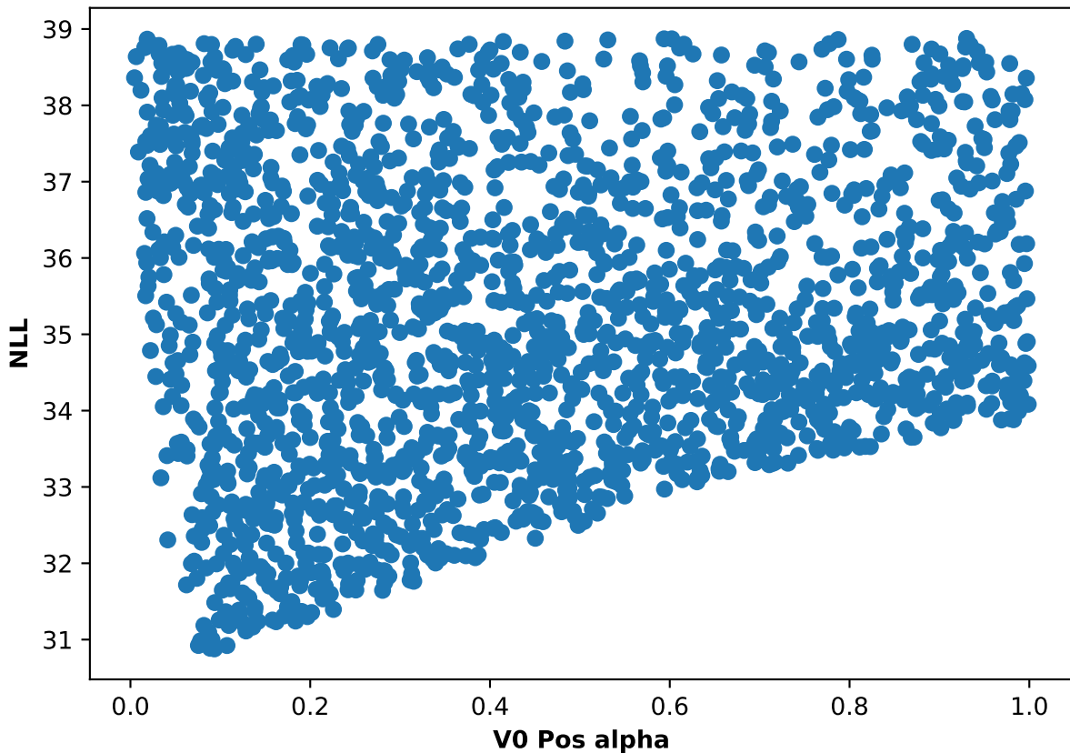
Participant 58, run 2: NLL and V0 Pos alpha scatter plot
