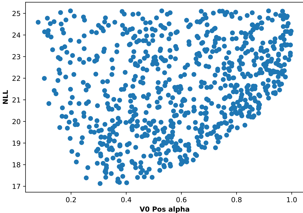
Participant 58, run 3: NLL and V0 Pos alpha scatter plot
