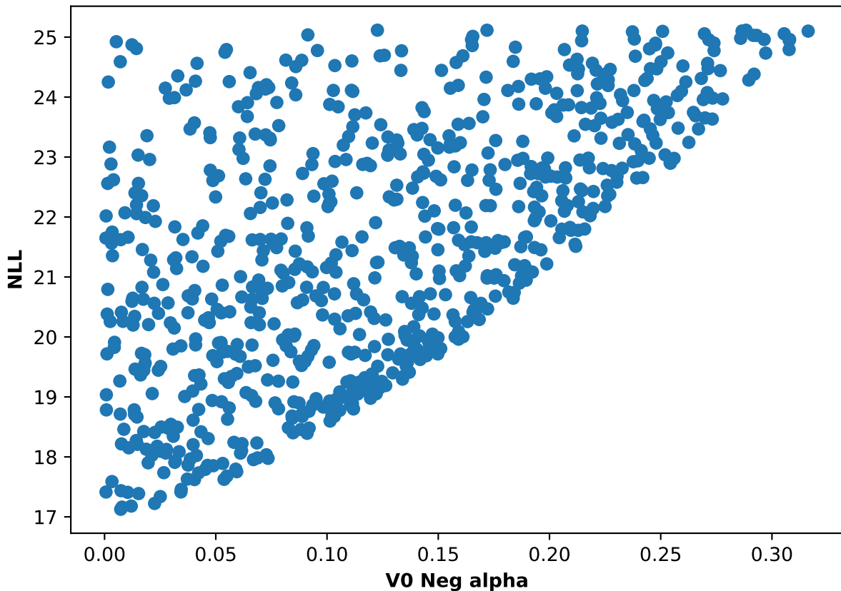
Participant 58, run 3: NLL and V0 Neg alpha scatter plot
