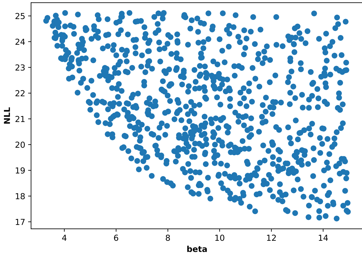
Participant 58, run 3: NLL and beta scatter plot
