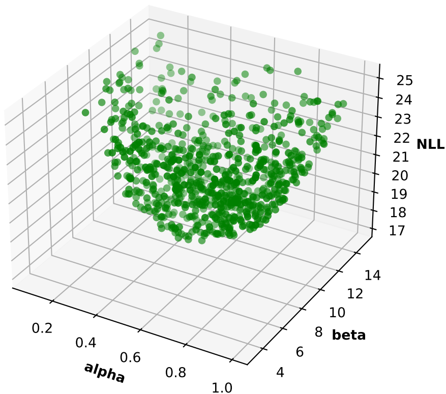
Participant 58, run 3: NLL, alpha and beta 3D scatter plot
