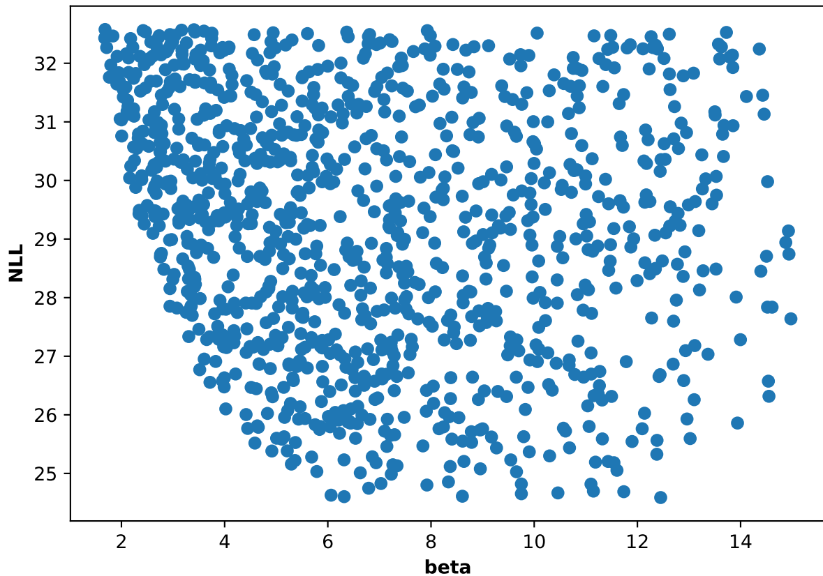
Participant 58, run 5: NLL and beta scatter plot
