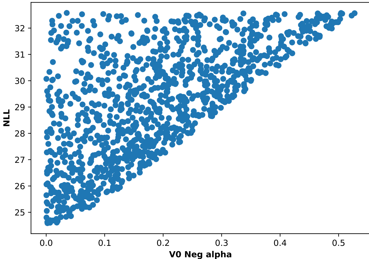
Participant 58, run 5: NLL and V0 Neg alpha scatter plot
