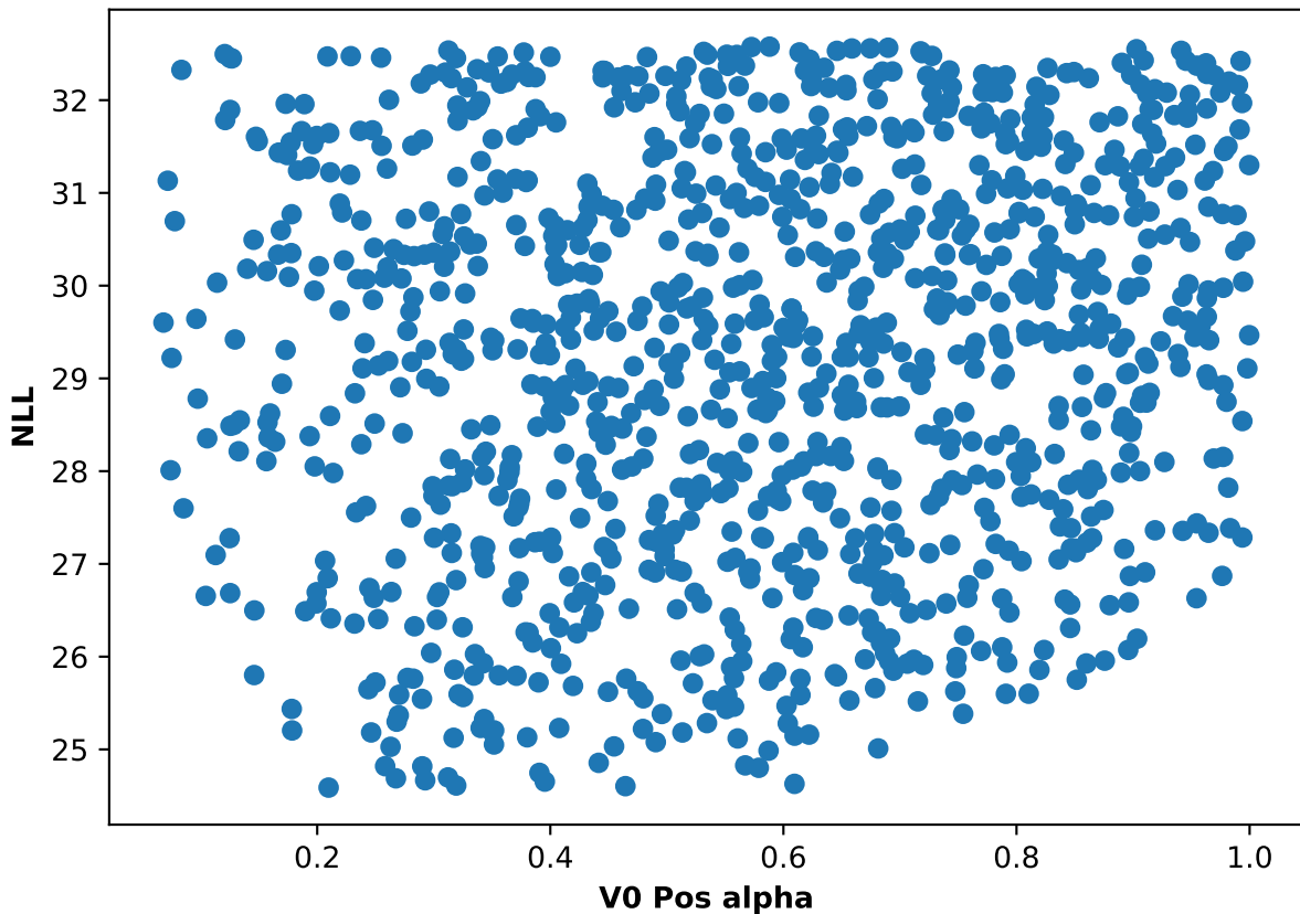
Participant 58, run 5: NLL and V0 Pos alpha scatter plot
