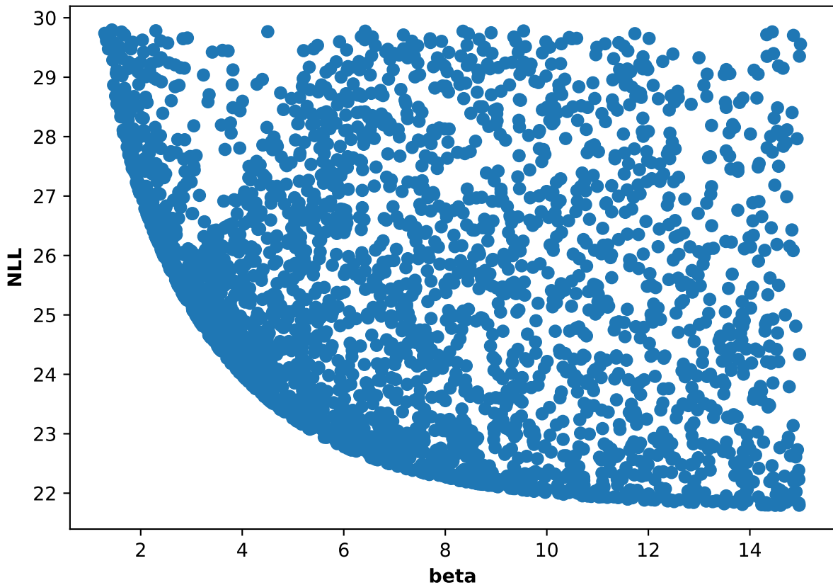
Participant 59, run 4: NLL and beta scatter plot
