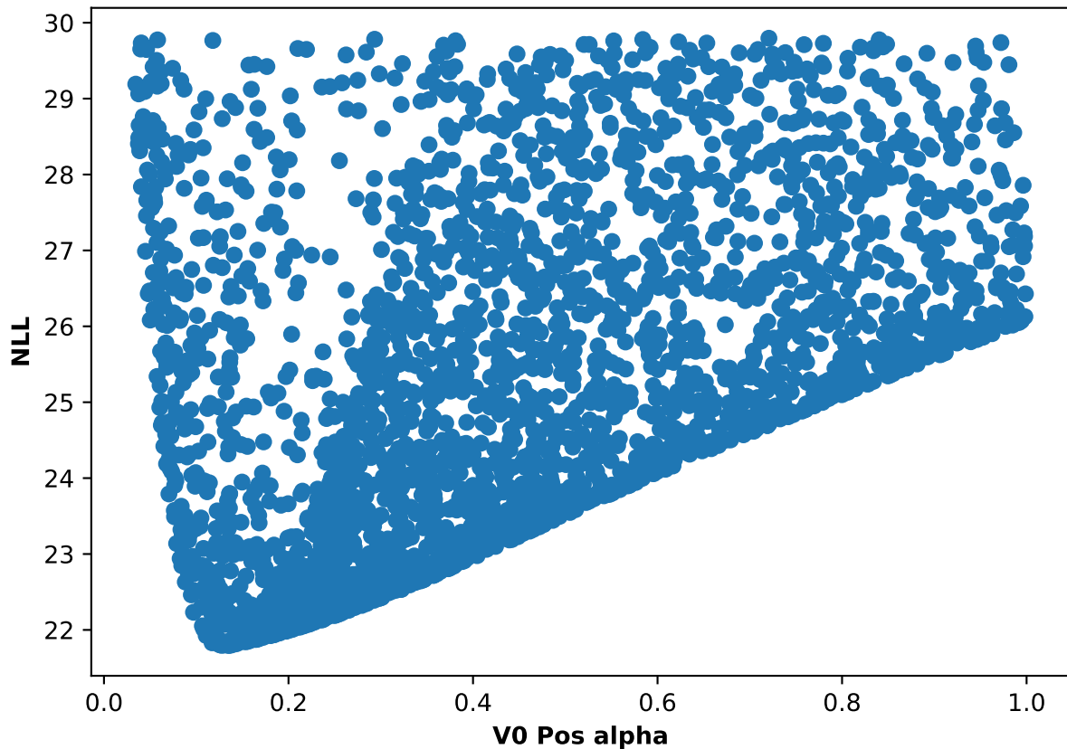
Participant 59, run 4: NLL and V0 Pos alpha scatter plot
