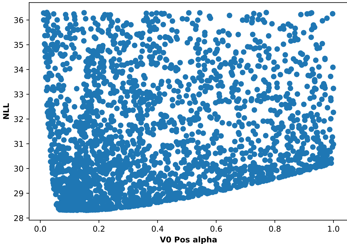
Participant 59, run 5: NLL and V0 Pos alpha scatter plot
