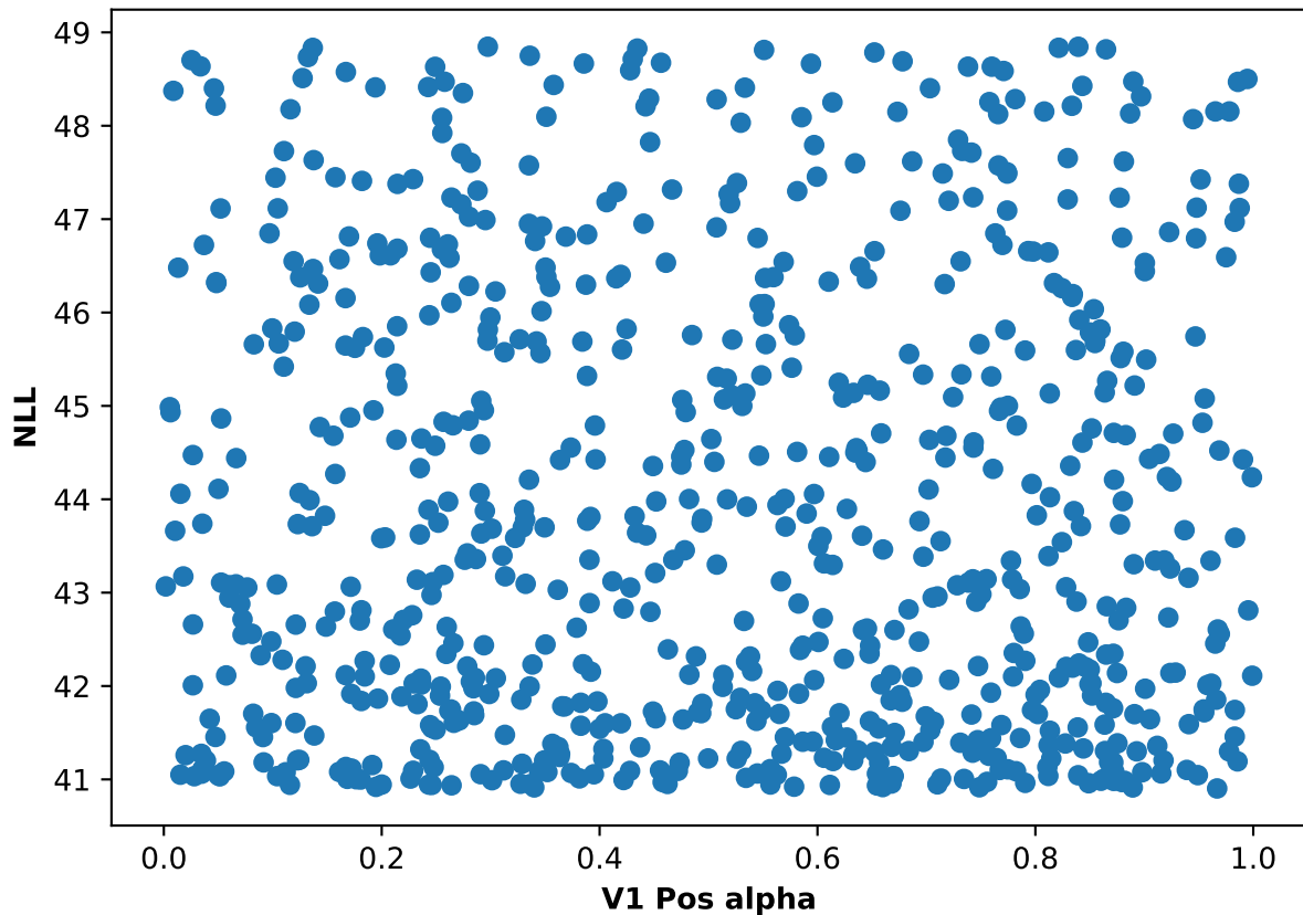
Participant 60, run 1: NLL and V1 Pos alpha scatter plot
