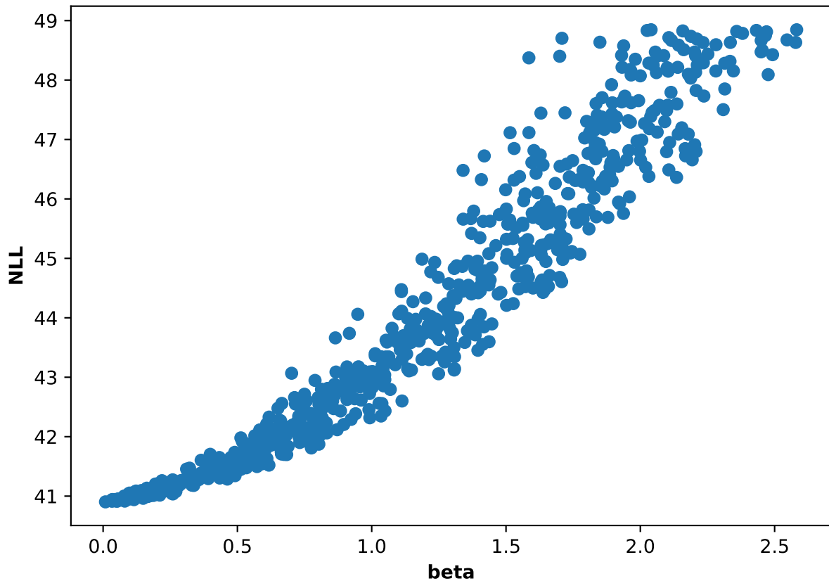
Participant 60, run 1: NLL and beta scatter plot
