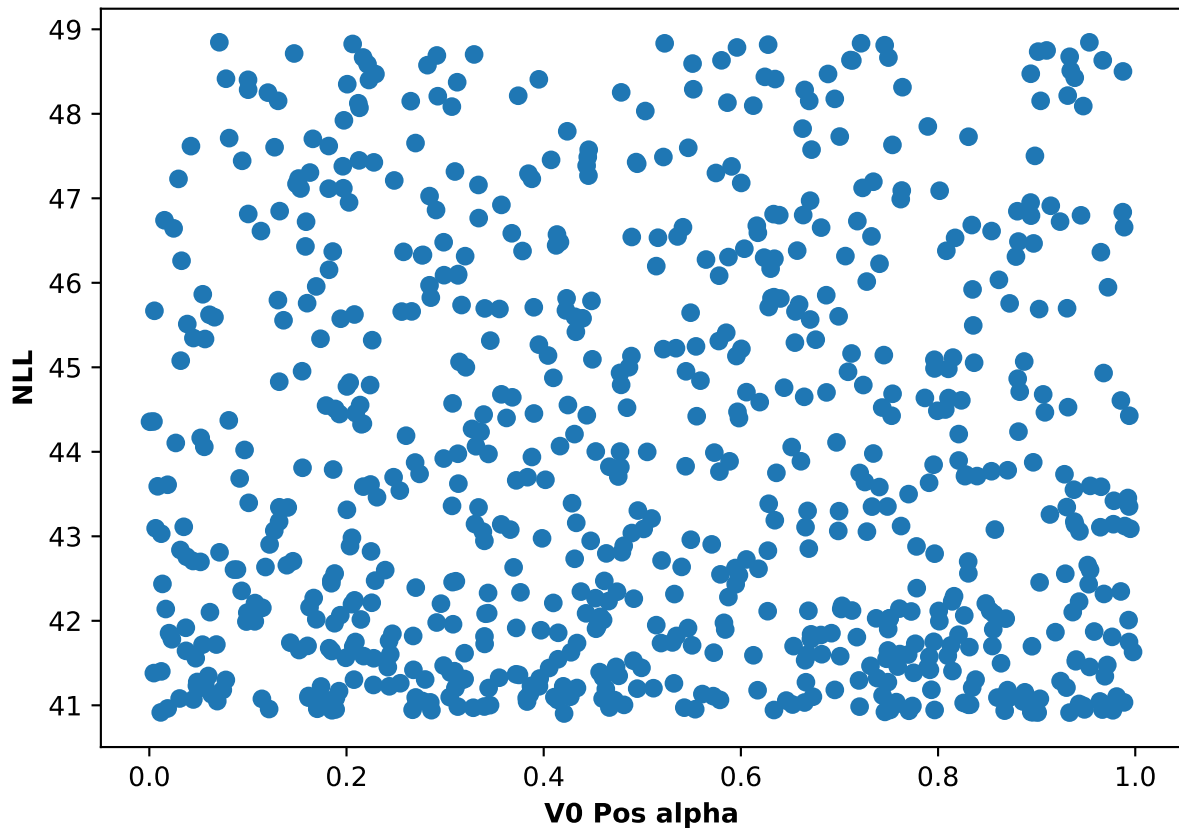
Participant 60, run 1: NLL and V0 Pos alpha scatter plot
