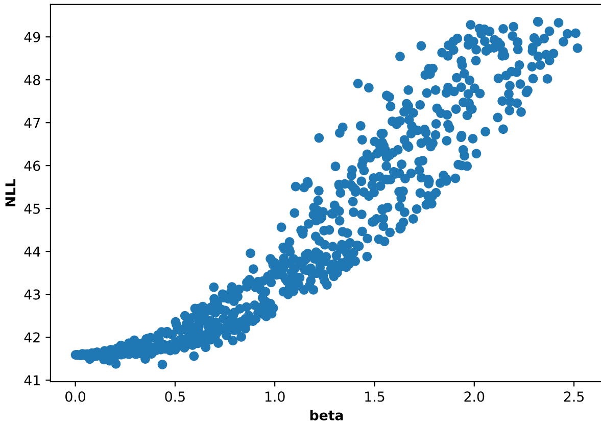
Participant 60, run 3: NLL and beta scatter plot
