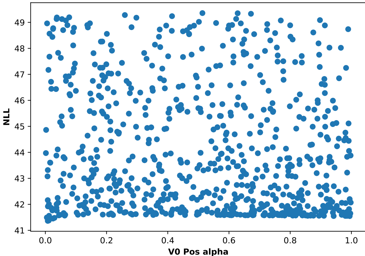
Participant 60, run 3: NLL and V0 Pos alpha scatter plot
