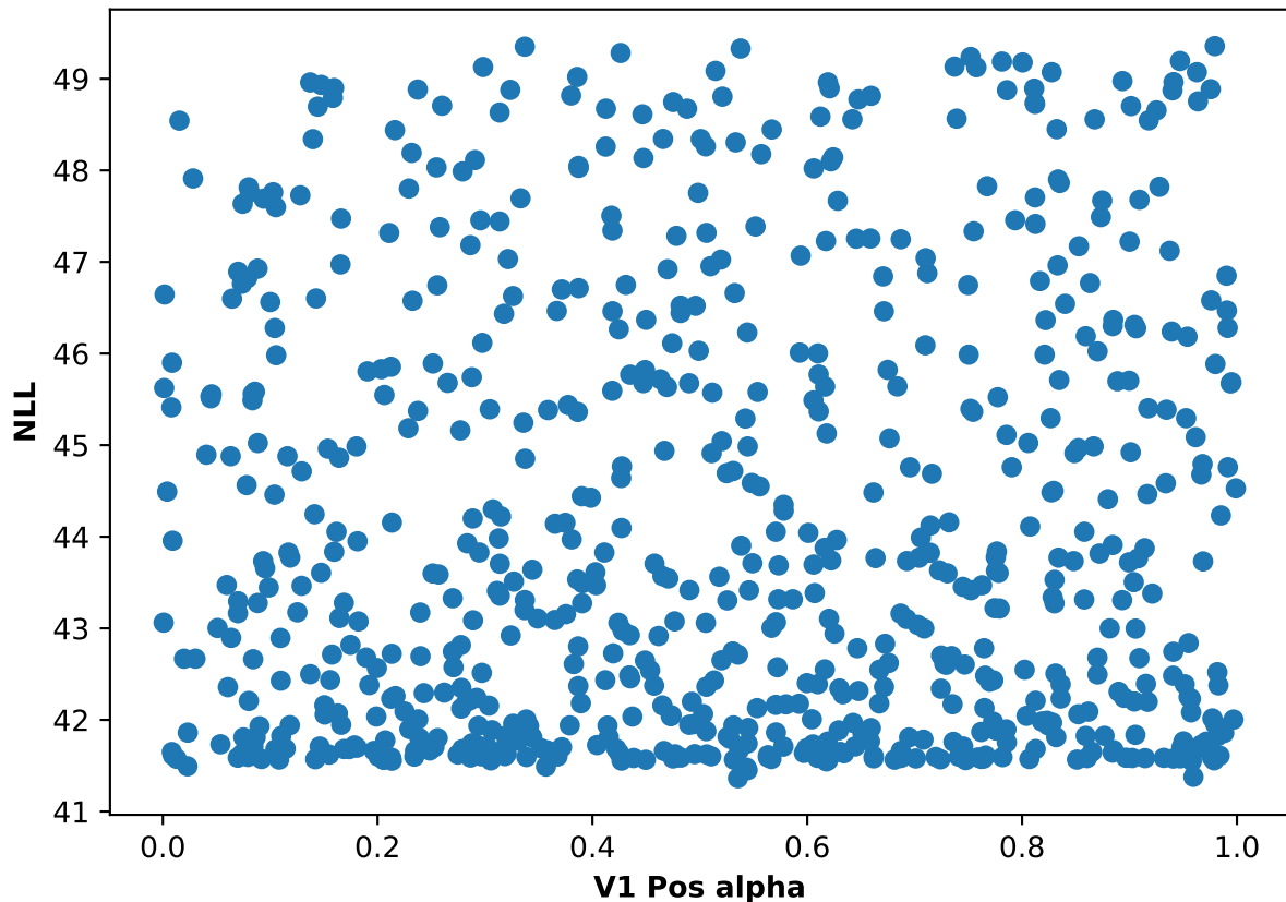
Participant 60, run 3: NLL and V1 Pos alpha scatter plot
