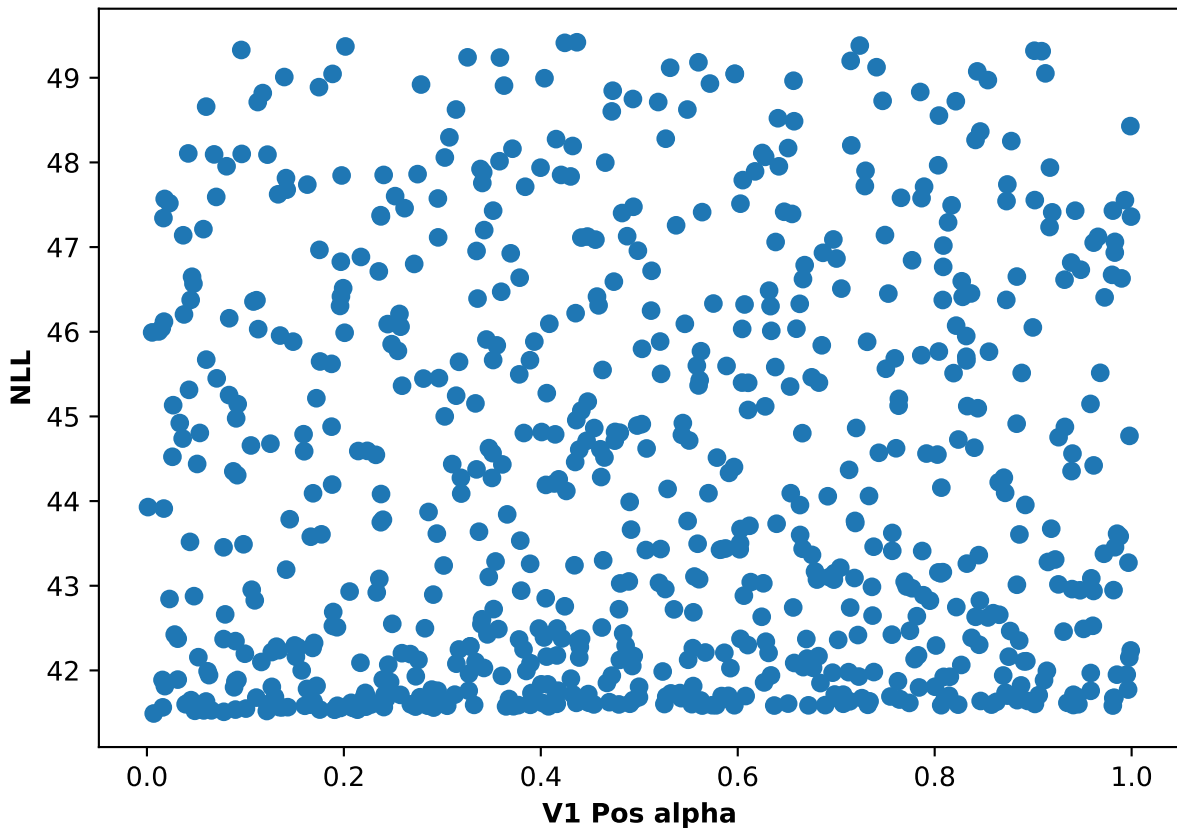
Participant 60, run 5: NLL and V1 Pos alpha scatter plot
