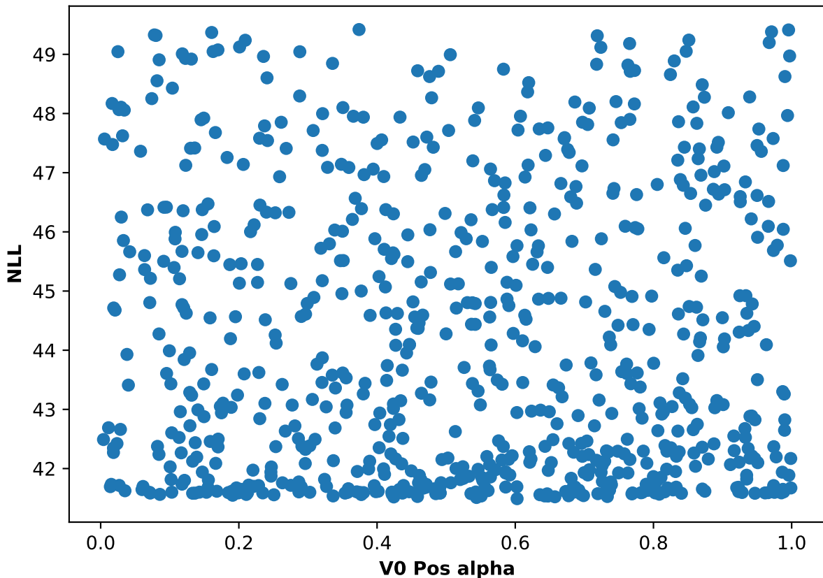
Participant 60, run 5: NLL and V0 Pos alpha scatter plot
