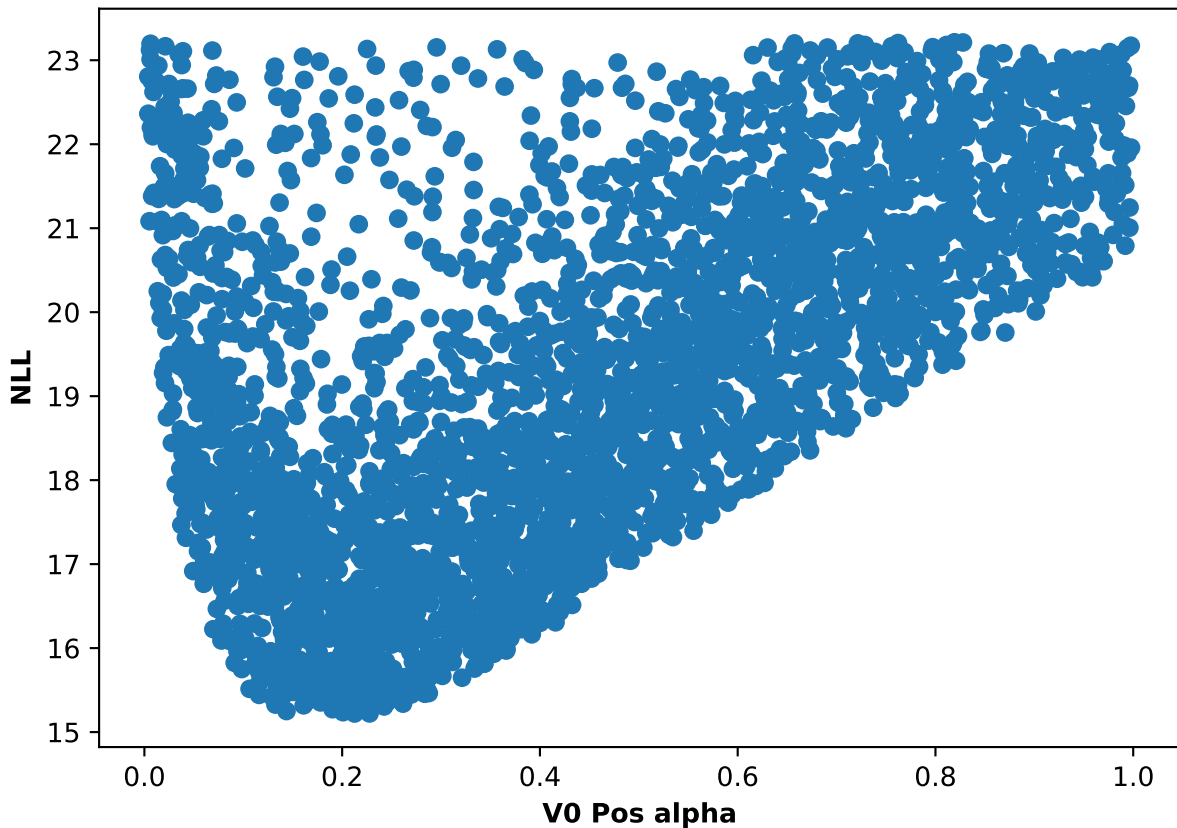
Participant 61, run 3: NLL and V0 Pos alpha scatter plot
