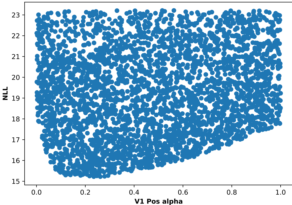
Participant 61, run 3: NLL and V1 Pos alpha scatter plot
