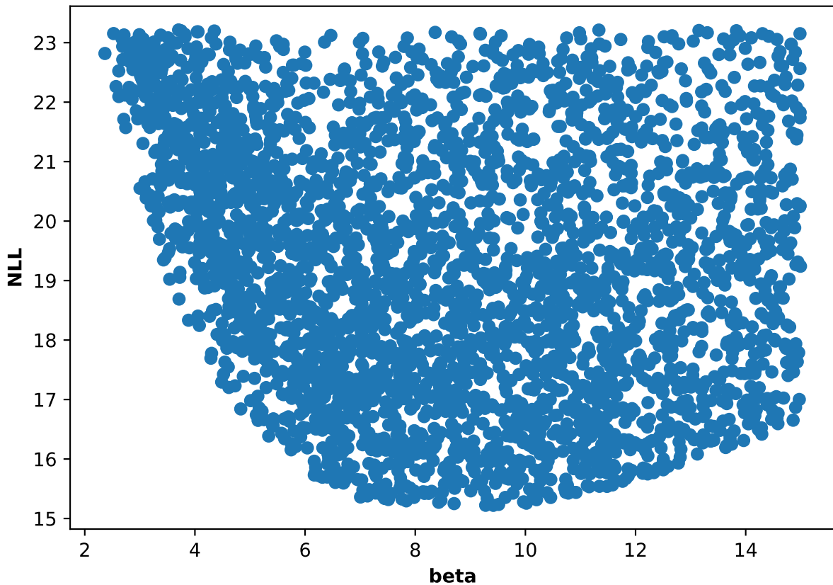
Participant 61, run 3: NLL and beta scatter plot
