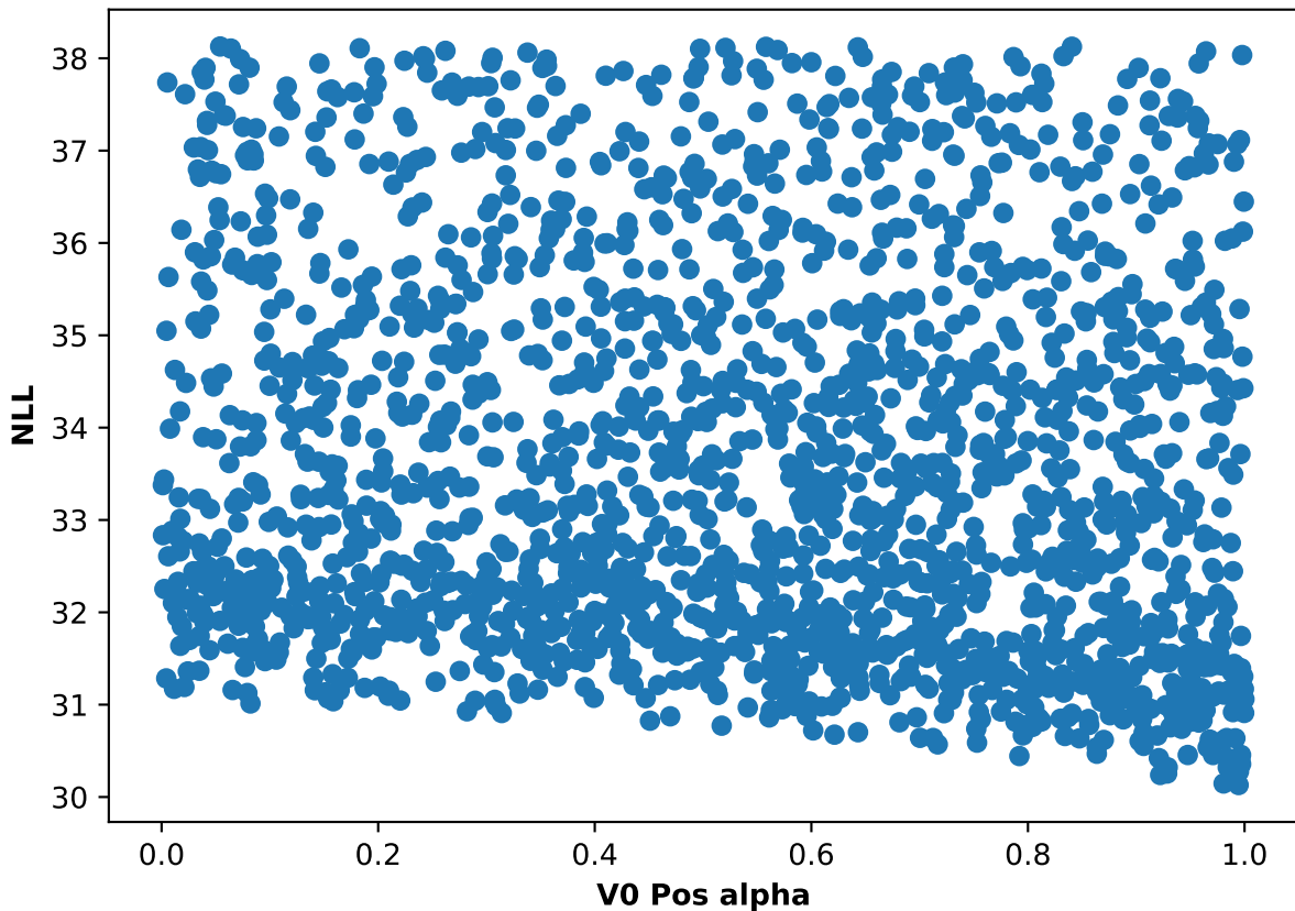
Participant 61, run 4: NLL and V0 Pos alpha scatter plot
