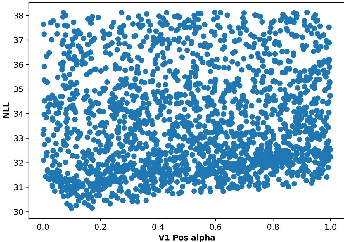
Participant 61, run 4: NLL and V1 Pos alpha scatter plot
