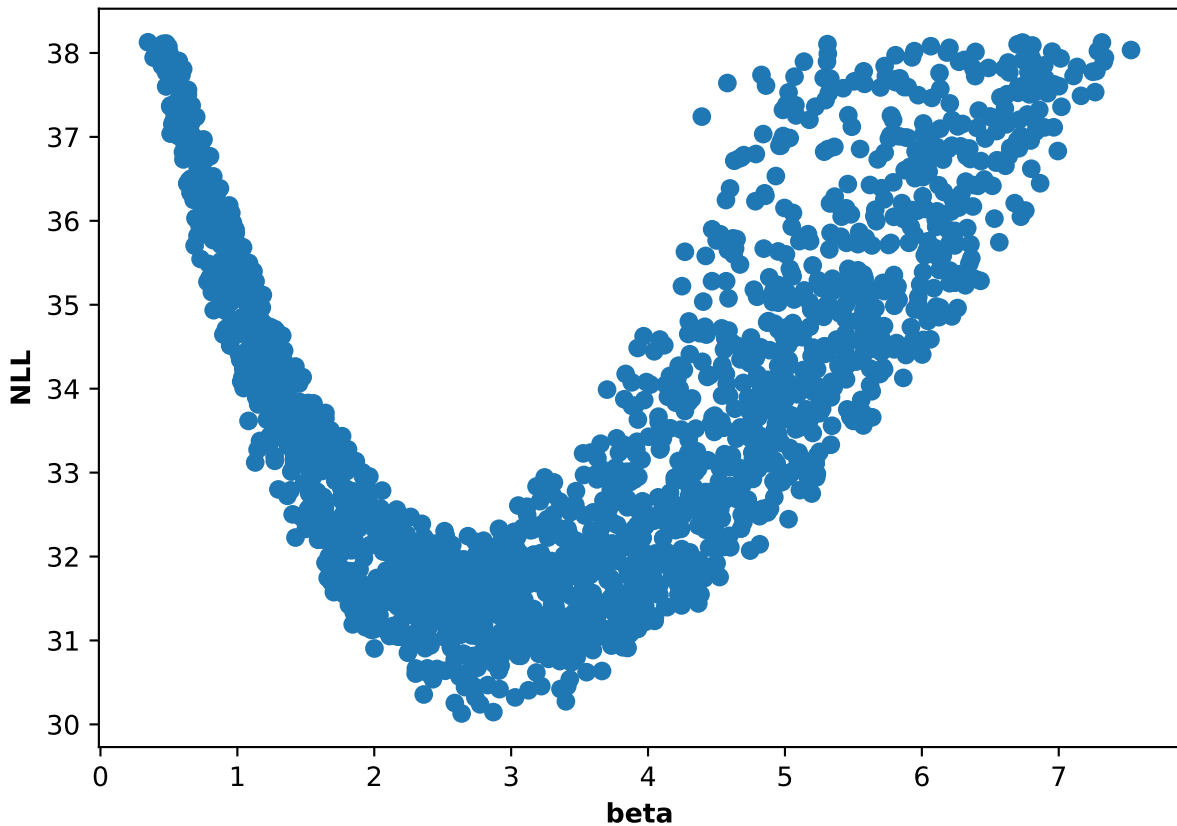
Participant 61, run 4: NLL and beta scatter plot
