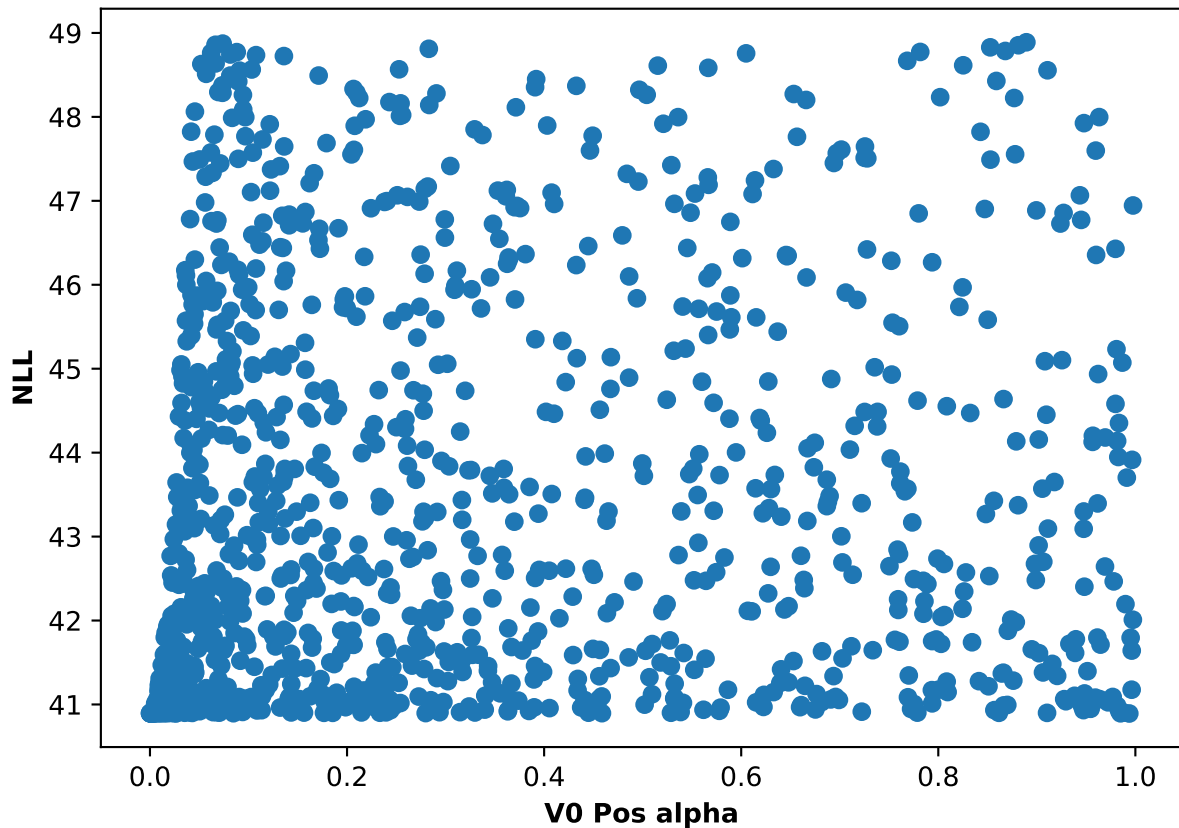
Participant 62, run 5: NLL and V0 Pos alpha scatter plot
