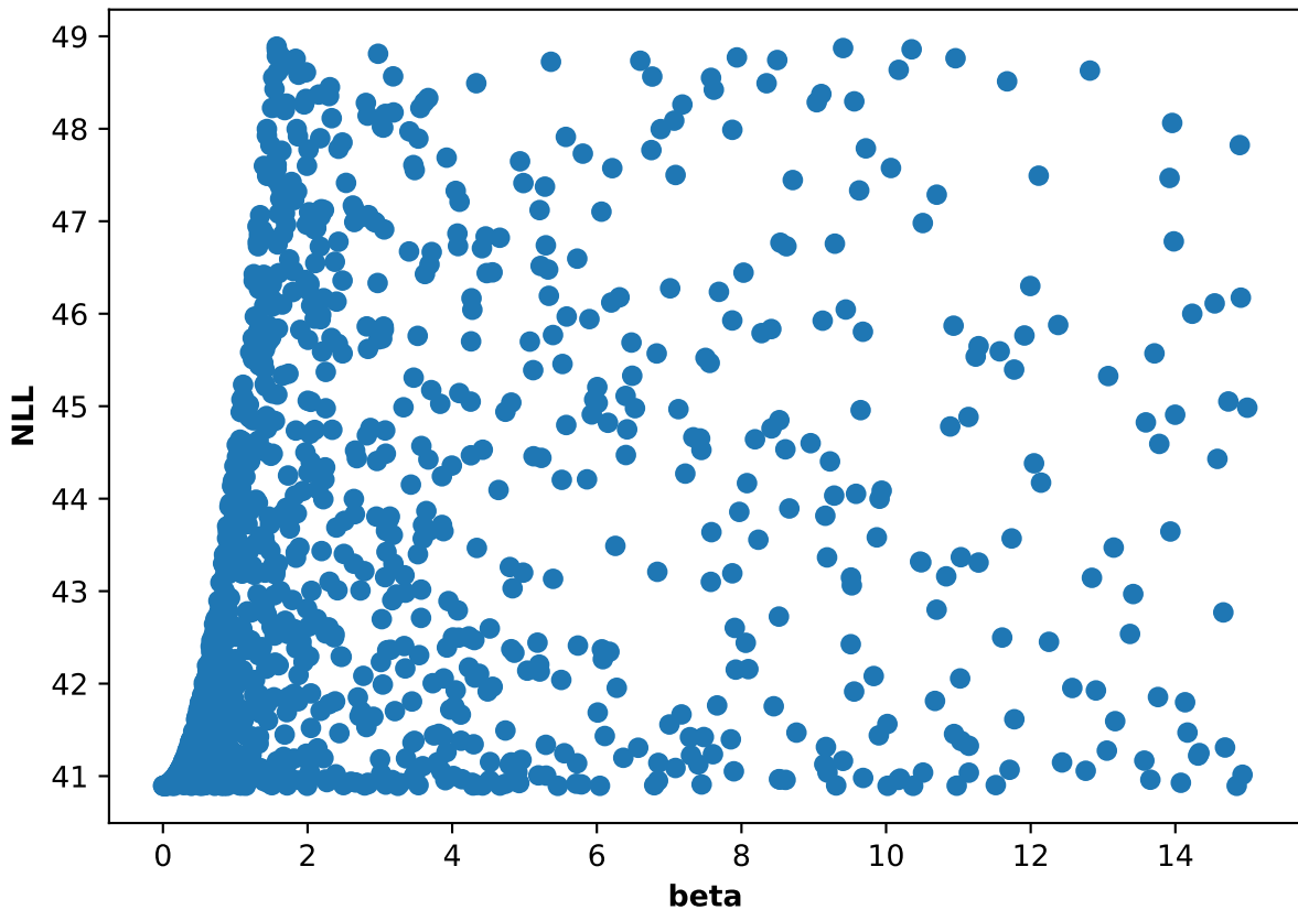
Participant 62, run 5: NLL and beta scatter plot
