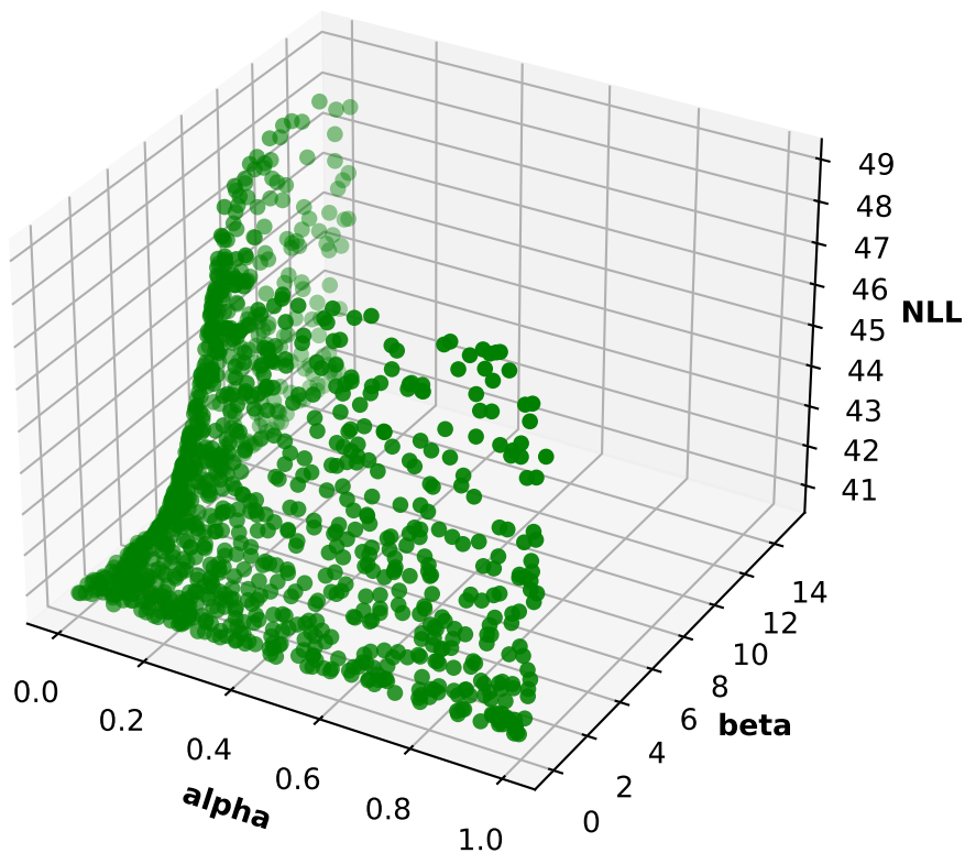
Participant 62, run 5: NLL, alpha and beta 3D scatter plot
