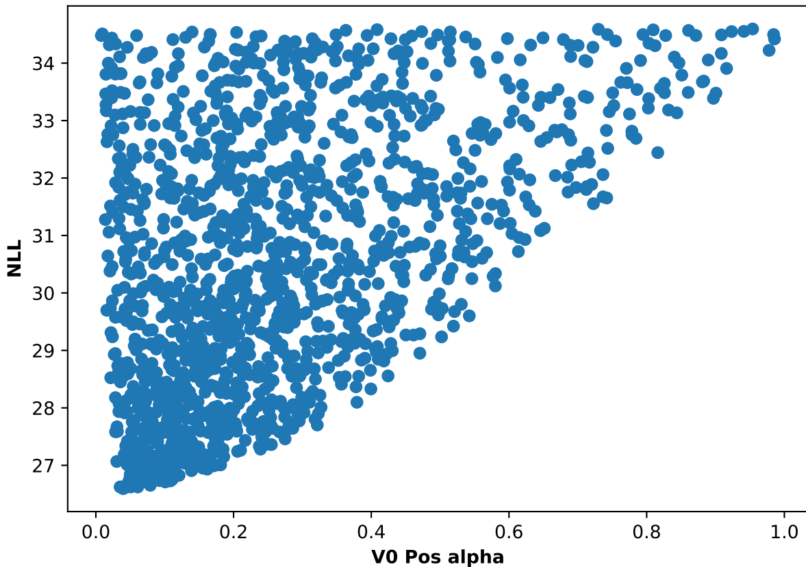
Participant 64, run 3: NLL and V0 Pos alpha scatter plot
