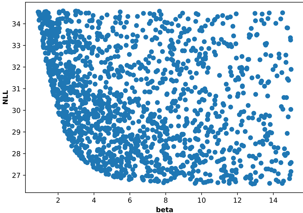
Participant 64, run 3: NLL and beta scatter plot
