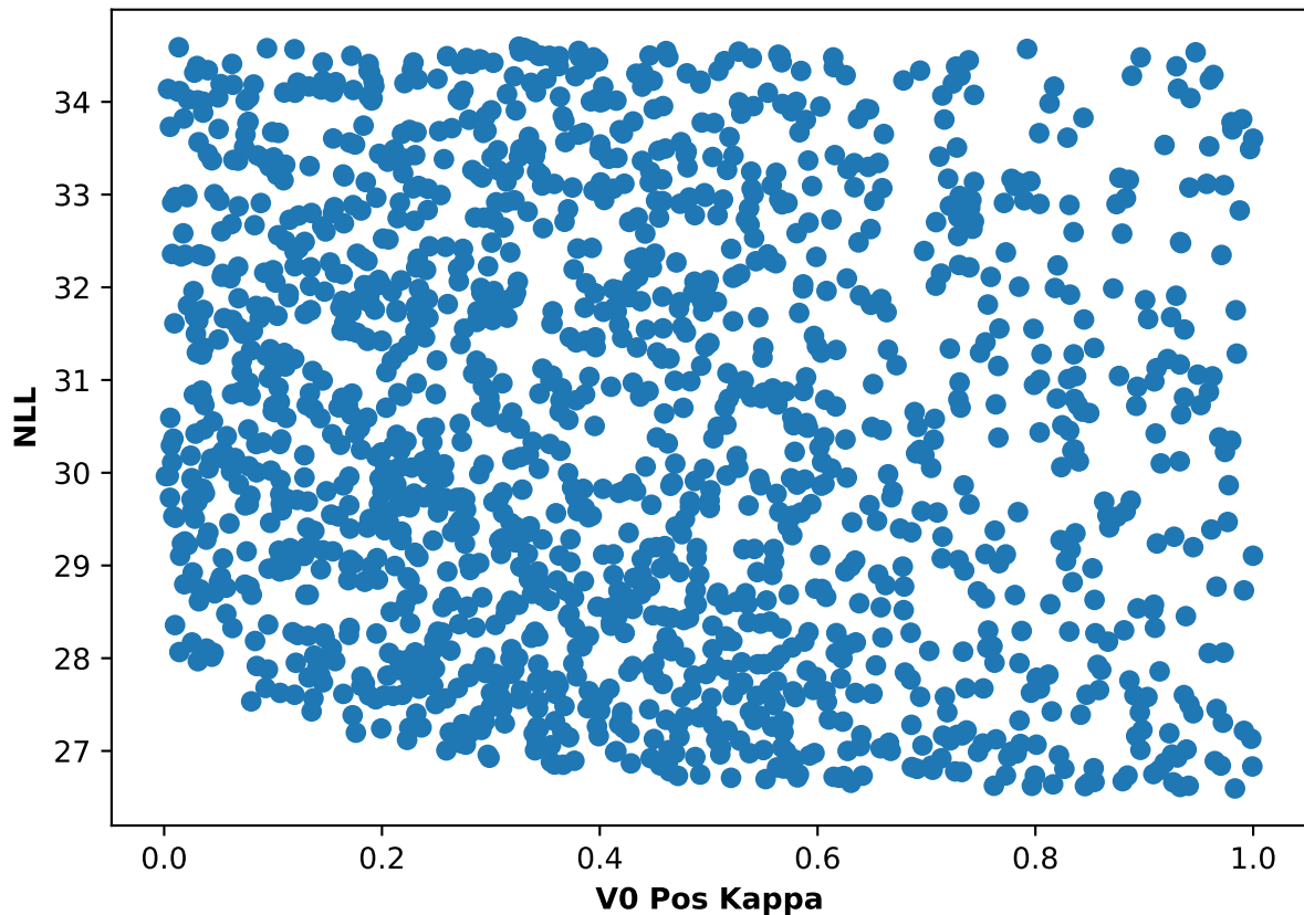
Participant 64, run 3: NLL and V0 Pos Kappa scatter plot
