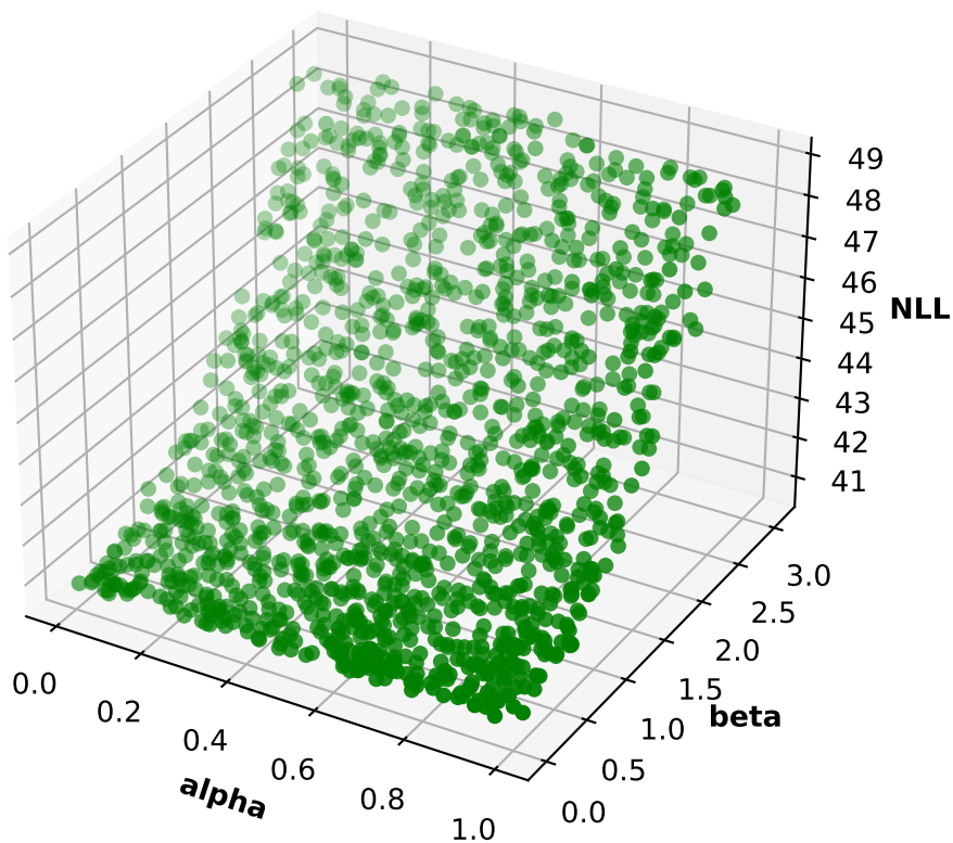
Participant 63, run 1: NLL, alpha and beta 3D scatter plot
