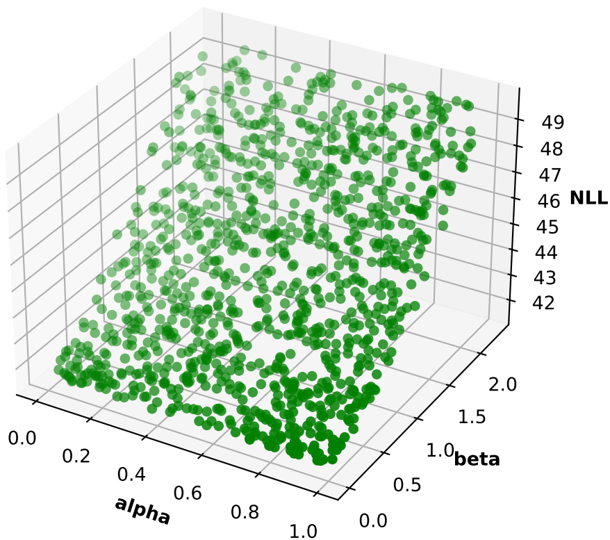
Participant 63, run 4: NLL, alpha and beta 3D scatter plot
