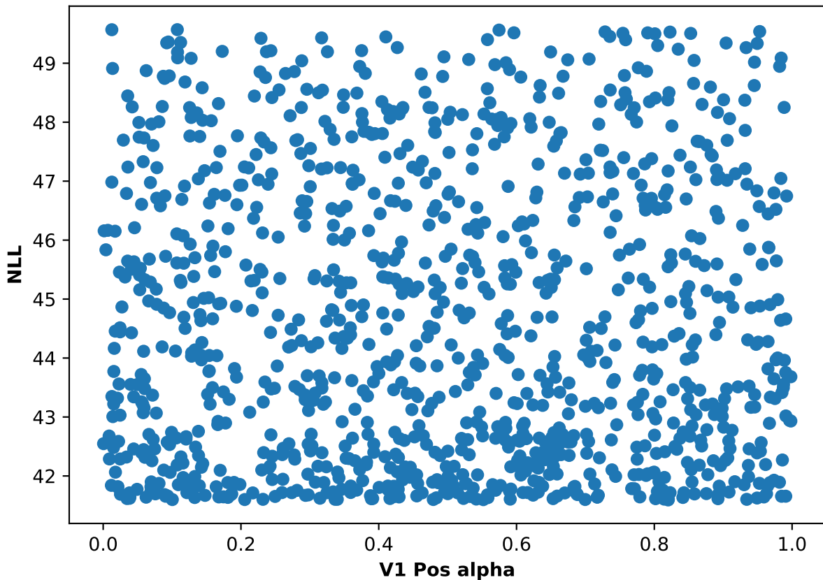
Participant 63, run 4: NLL and V1 Pos alpha scatter plot
