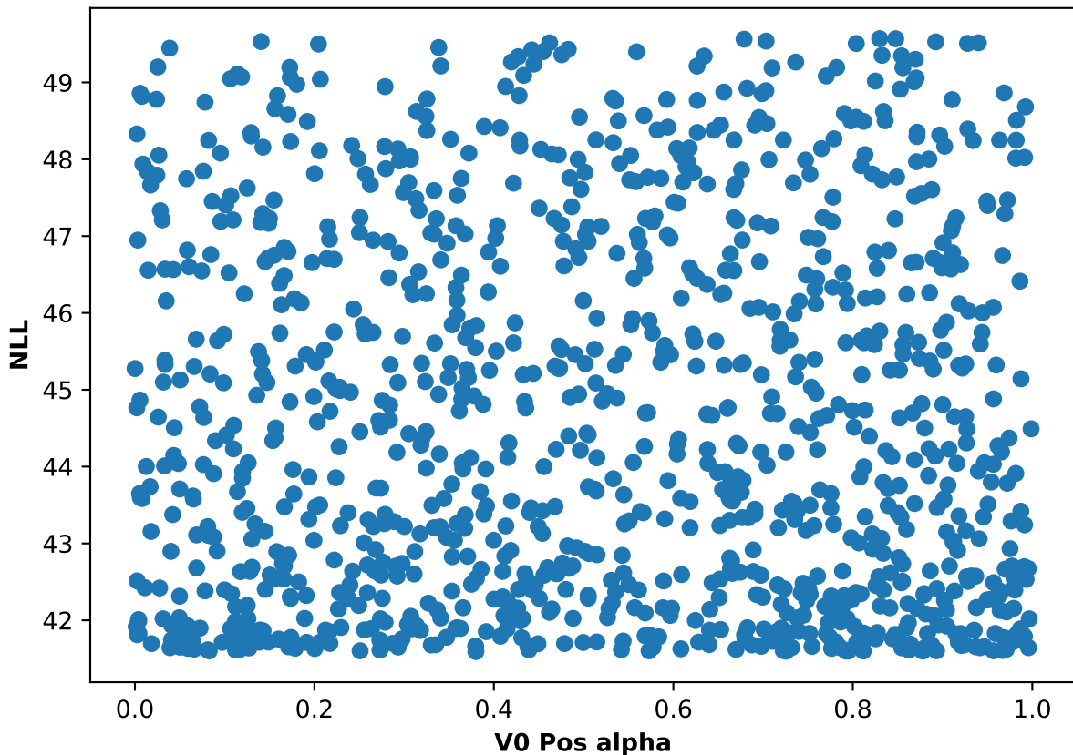
Participant 63, run 4: NLL and V0 Pos alpha scatter plot
