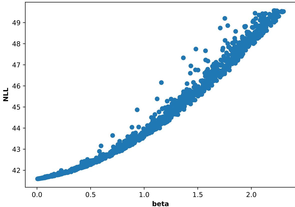
Participant 63, run 4: NLL and beta scatter plot
