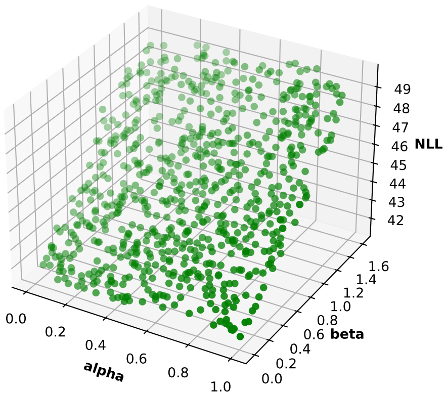
Participant 63, run 5: NLL, alpha and beta 3D scatter plot
