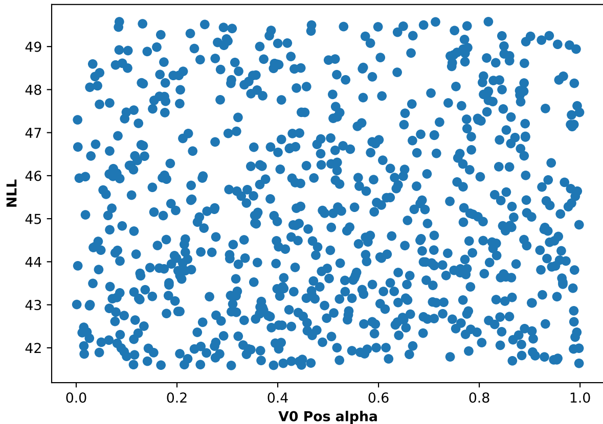
Participant 63, run 5: NLL and V0 Pos alpha scatter plot
