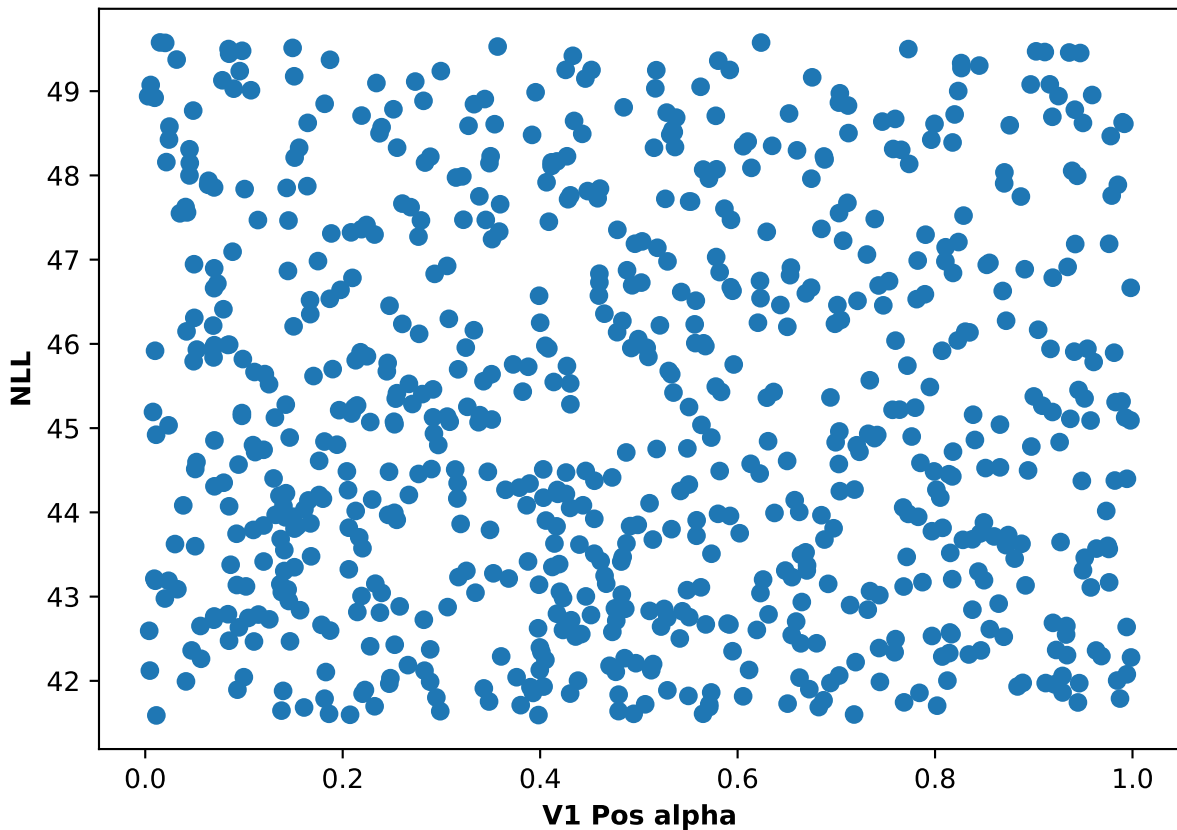
Participant 63, run 5: NLL and V1 Pos alpha scatter plot
