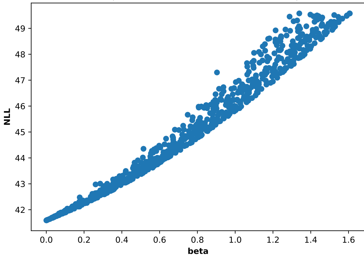
Participant 63, run 5: NLL and beta scatter plot
