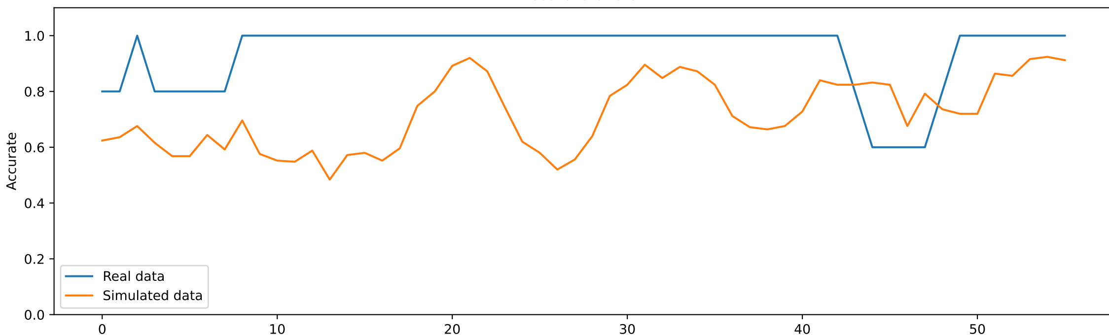
Accurate overall
