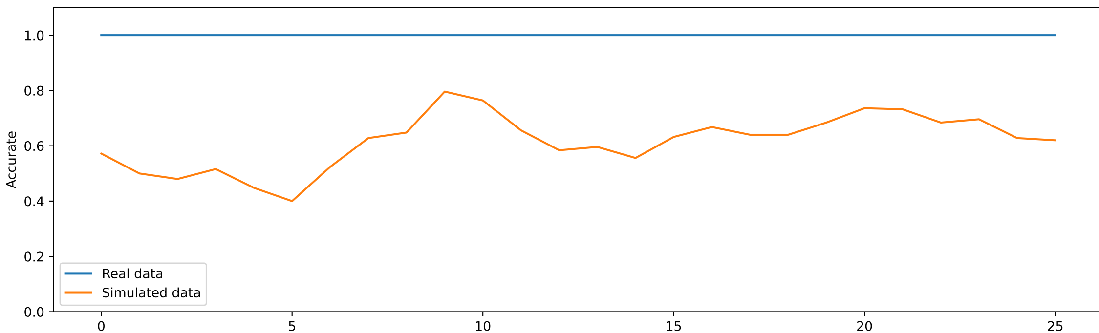
Accurate overall
