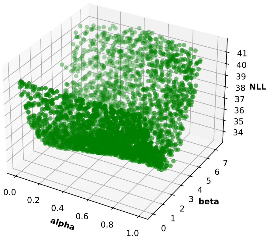
Participant 64, run 3: NLL, alpha and beta 3D scatter plot
