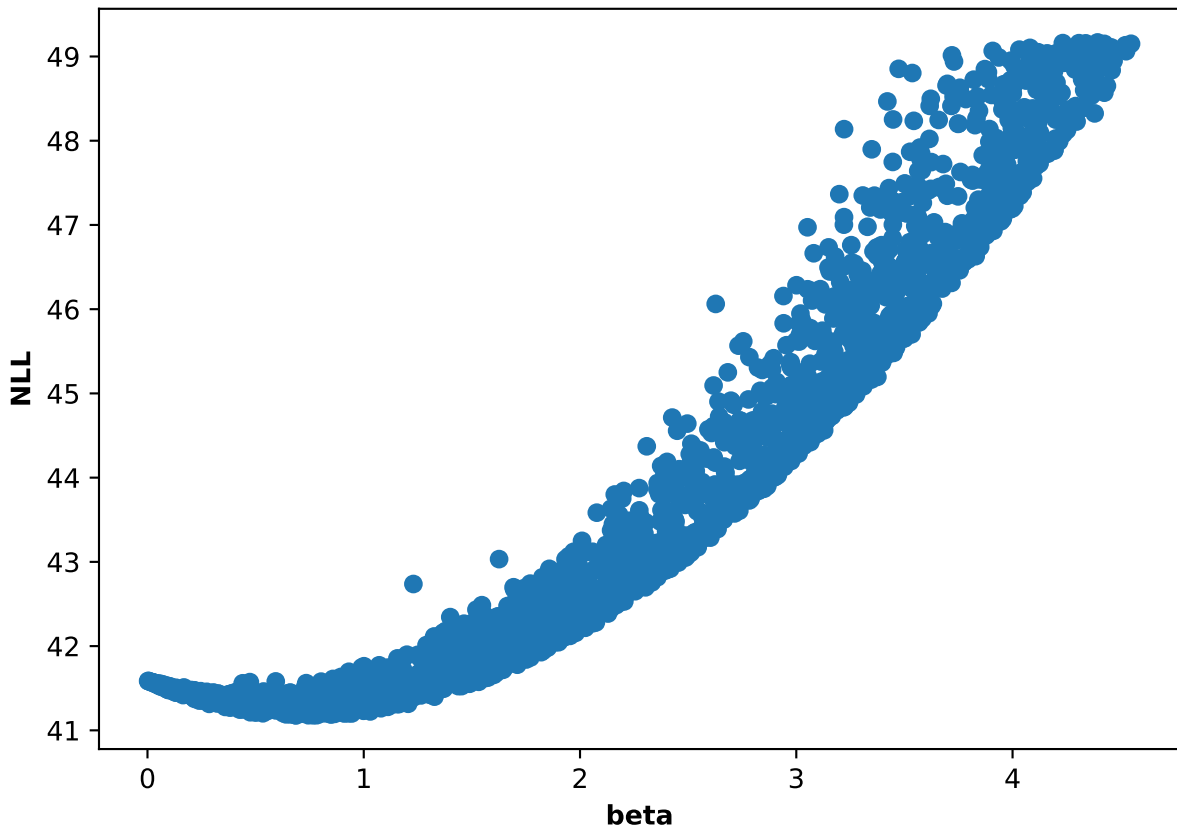
Participant 64, run 4: NLL and beta scatter plot
