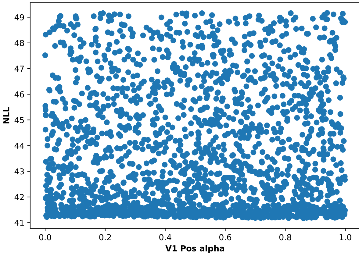
Participant 64, run 4: NLL and V1 Pos alpha scatter plot
