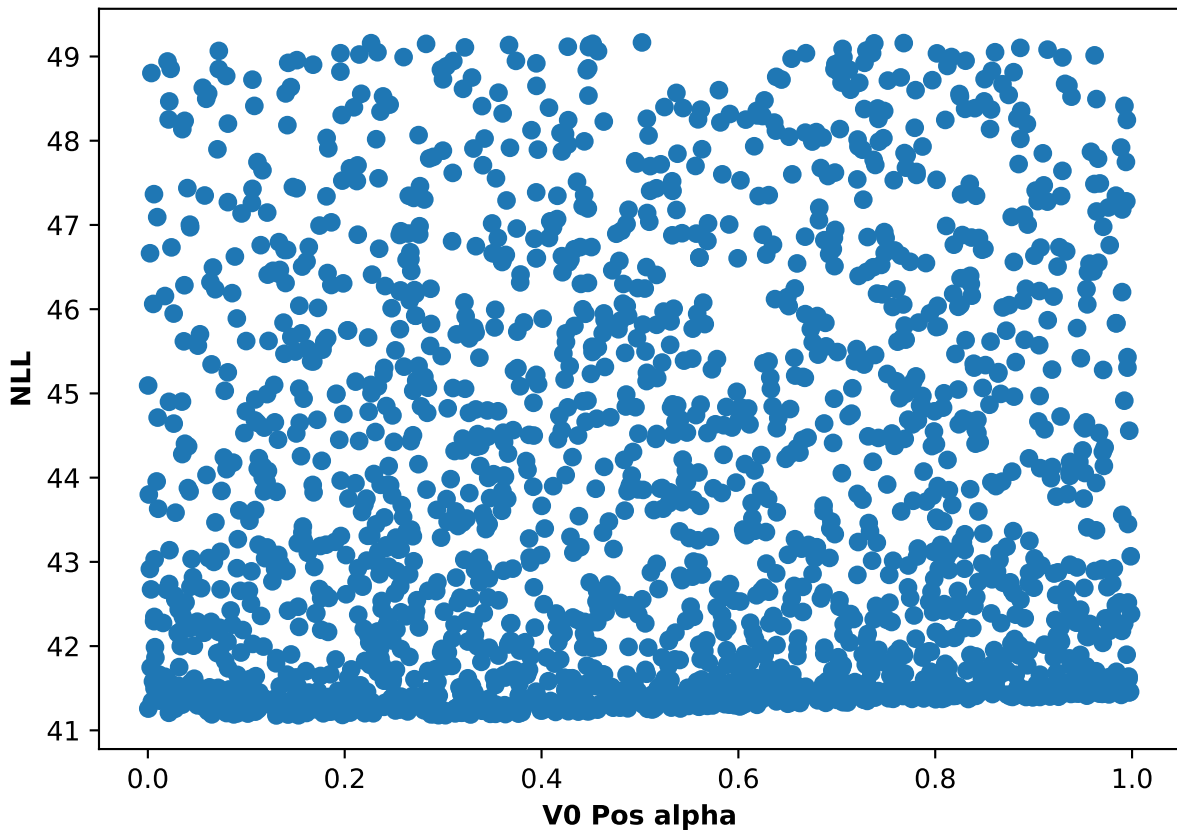
Participant 64, run 4: NLL and V0 Pos alpha scatter plot
