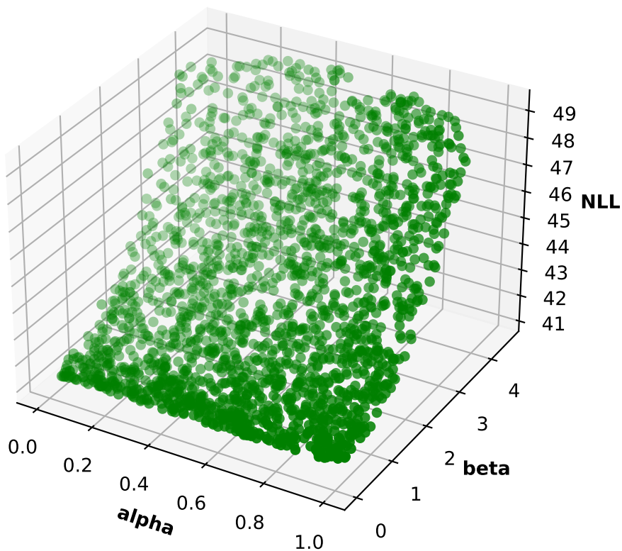
Participant 64, run 4: NLL, alpha and beta 3D scatter plot
