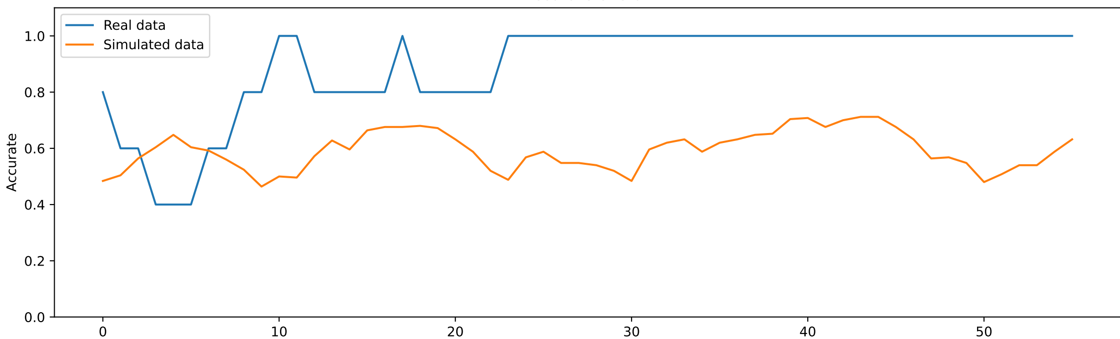
Accurate overall
