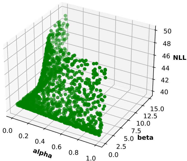
Participant 15, run 3: NLL, alpha and beta 3D scatter plot
