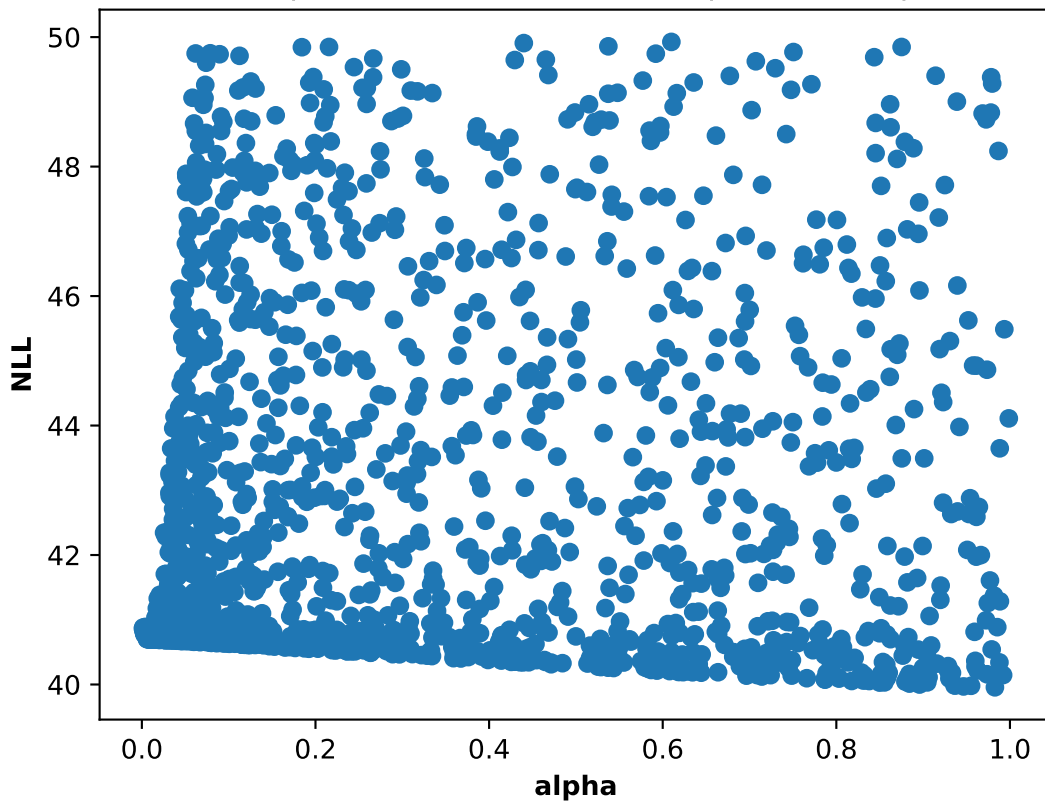
Participant 15, run 3: NLL and alpha scatter plot
