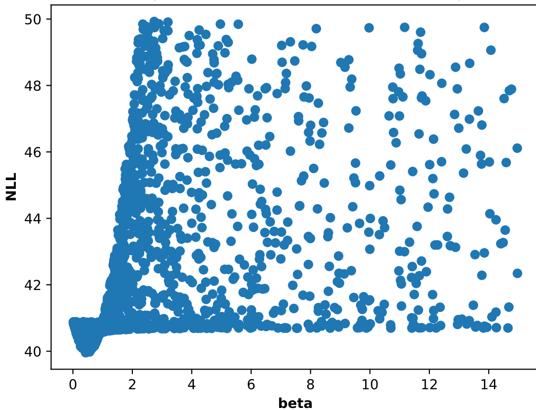
Participant 15, run 3: NLL and beta scatter plot
