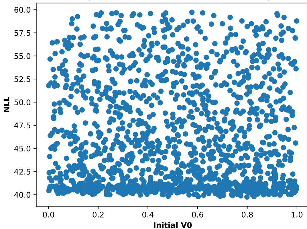
Participant 15, run 3: NLL and Init V0 scatter plot
