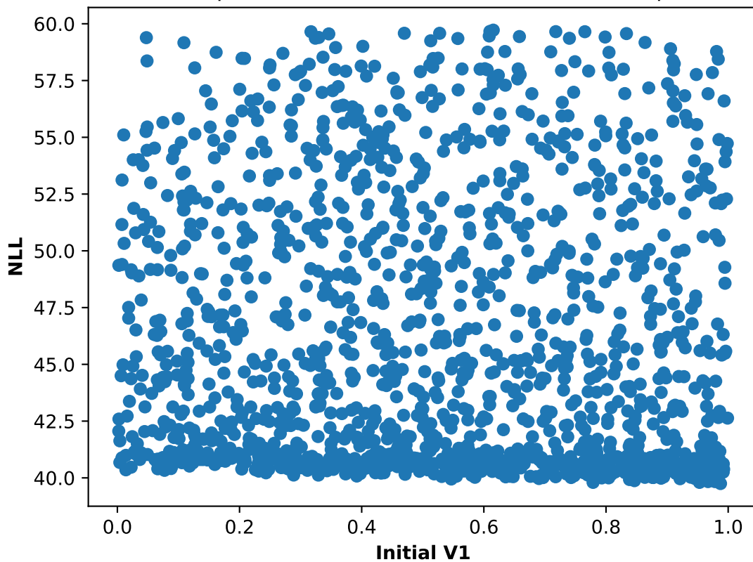
Participant 15, run 3: NLL and Init V1 scatter plot
