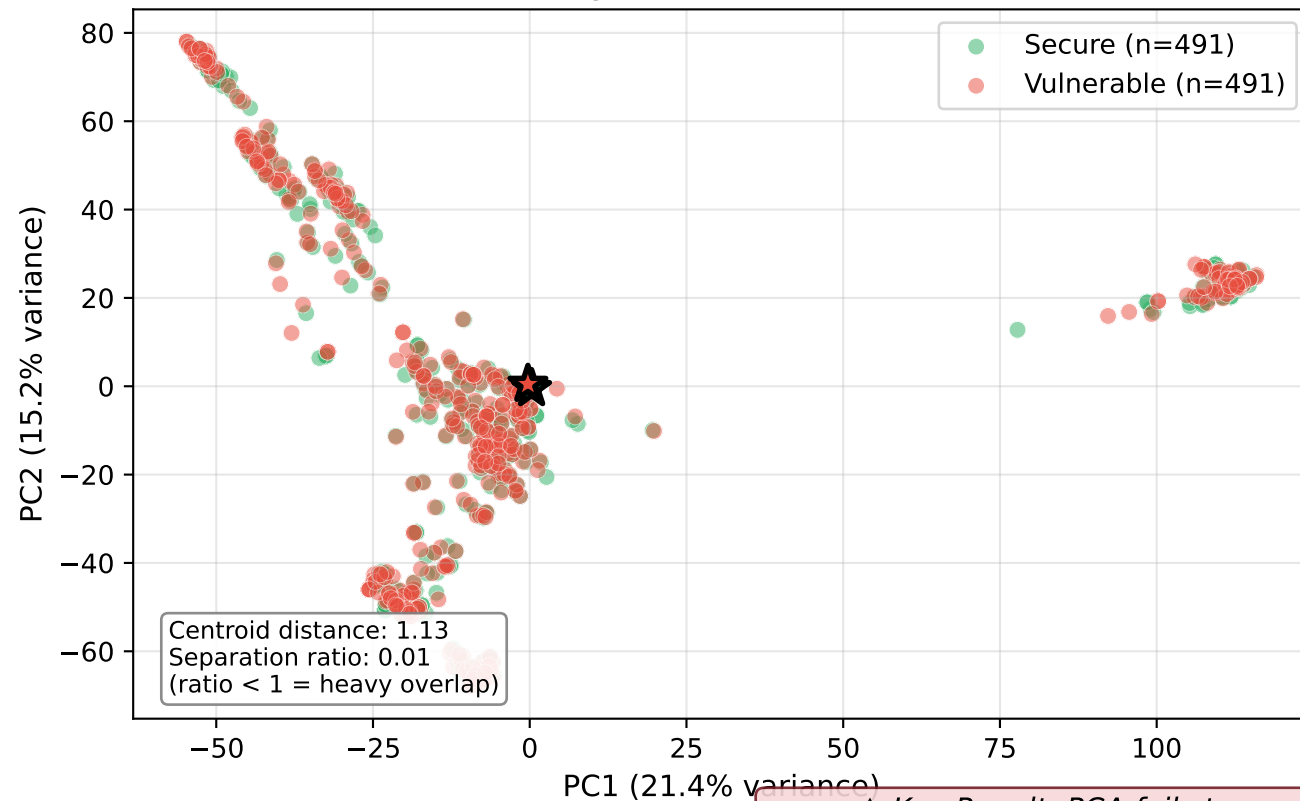
PCA Projection of SAE Latents
