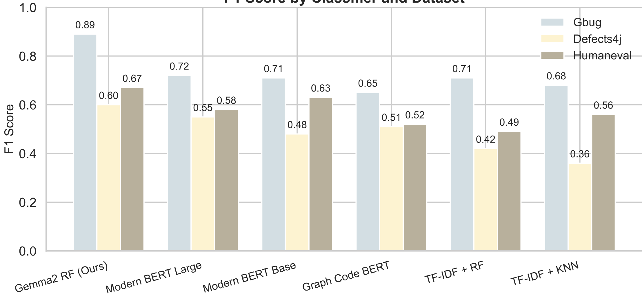
F1 Score by Classifier and Dataset
