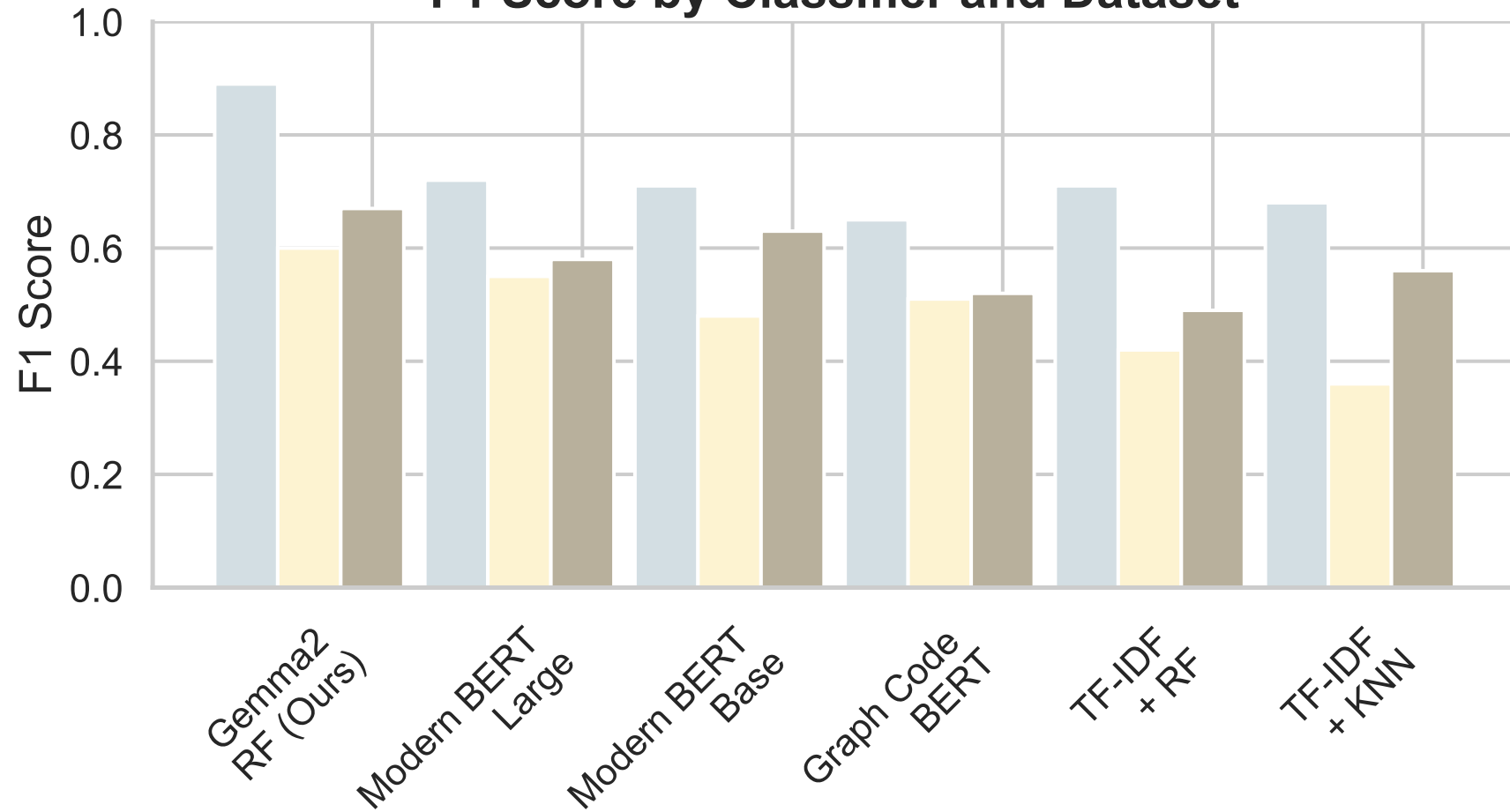
F1 Score by Classifier and Dataset
