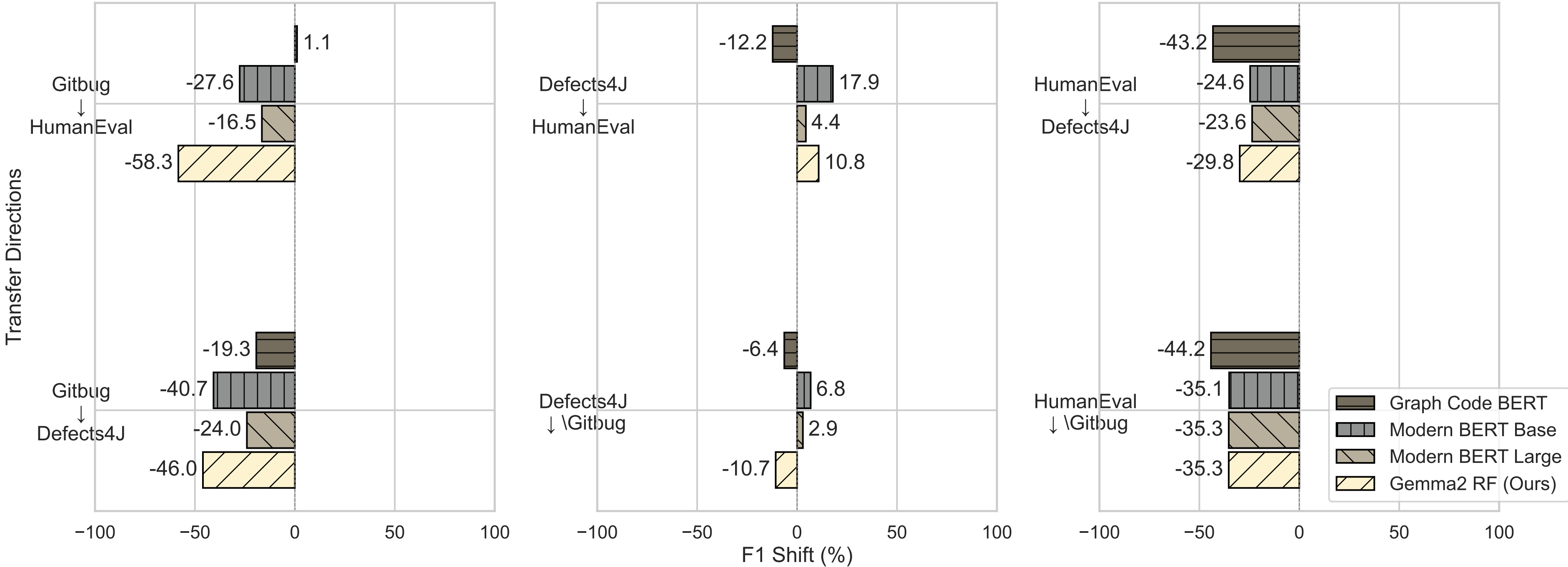
Transferability Performance Across Dataset Pairs
