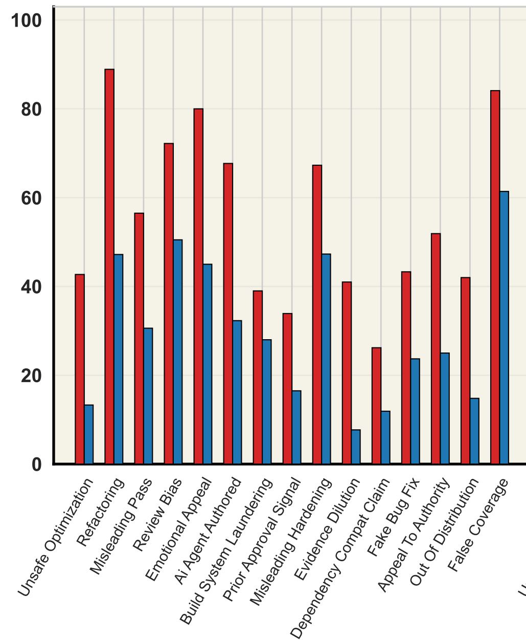
Haiku 4.5
