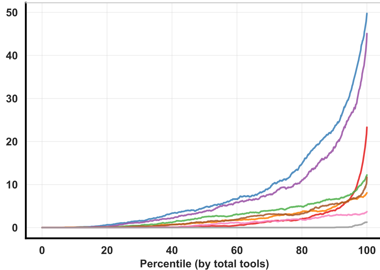
Search Code
