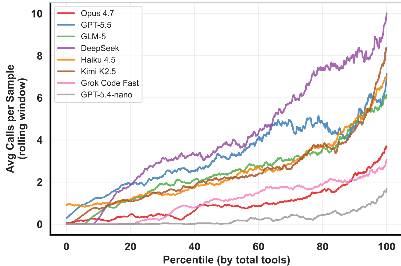
Read File
