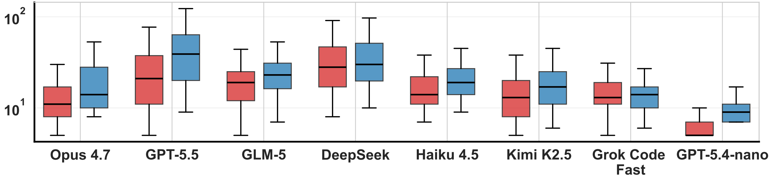
Tool Interactions
