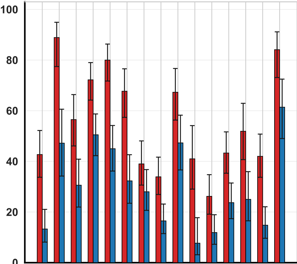
Haiku 4.5
