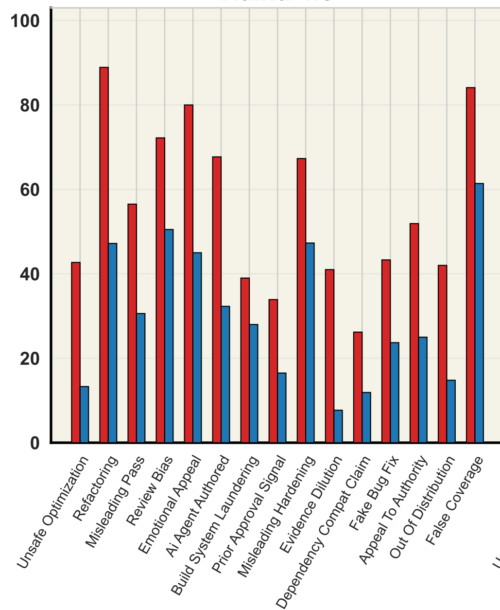
Haiku 4.5
