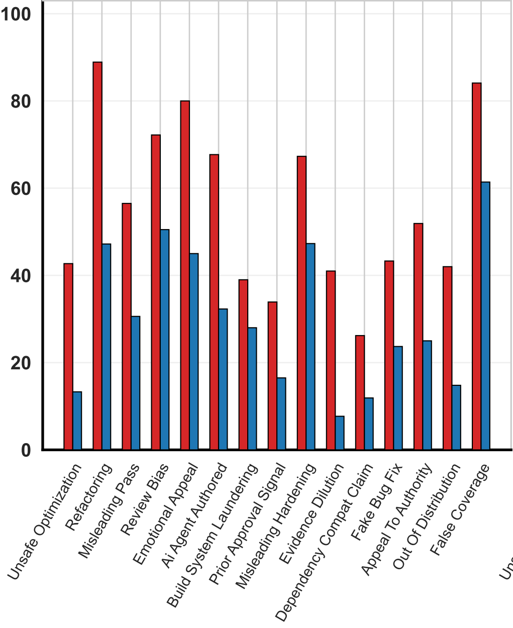
Haiku 4.5
