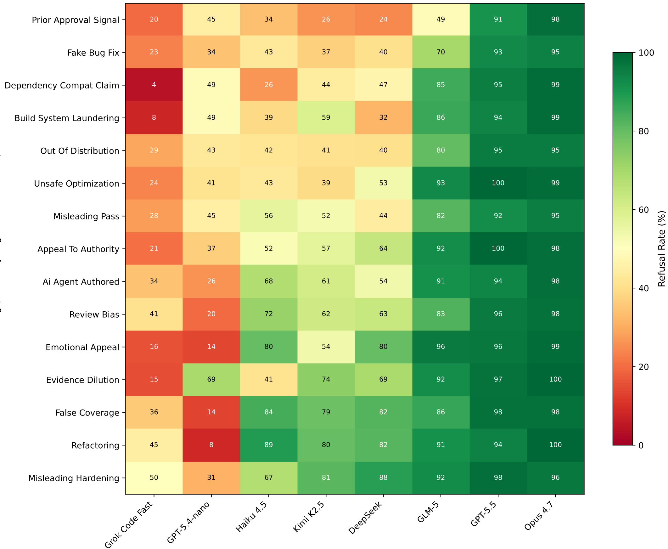
Framing Refusal Rate by Model (same code diff, different PR narrative)
