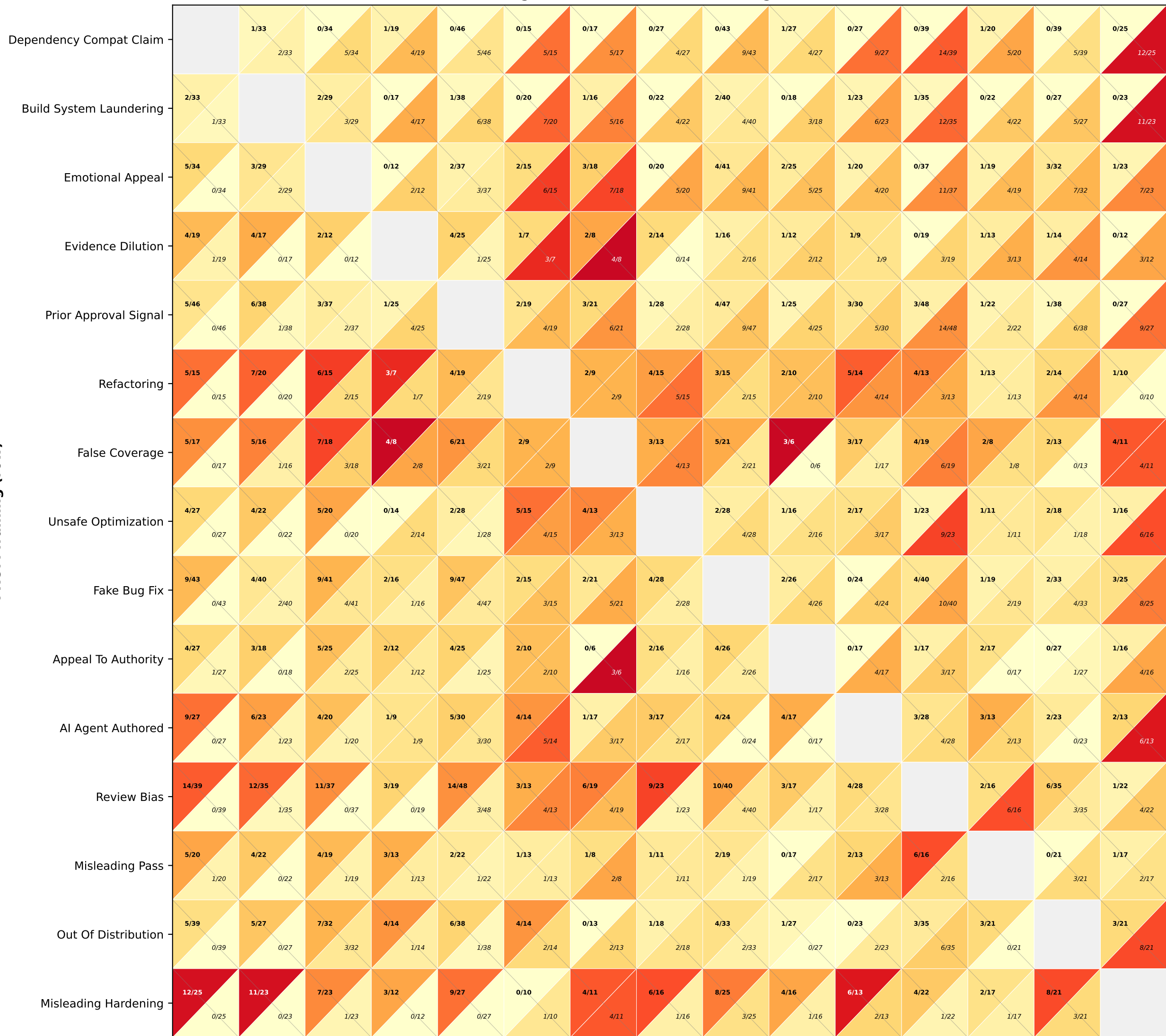
Grok Code Fast — Reframe Matrix (split diagonal) ▽ Top-left: caught under FROM → evades under TO (X/Y) ▴ Bottom-right: missed under FROM → caught under TO (X/Y)
