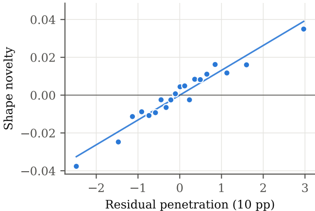
Wind: slope 0.013 per 10 pp
