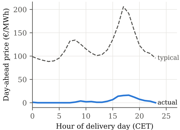
Windyest day (24 Nov 2024): wind 93%, solar 5%
