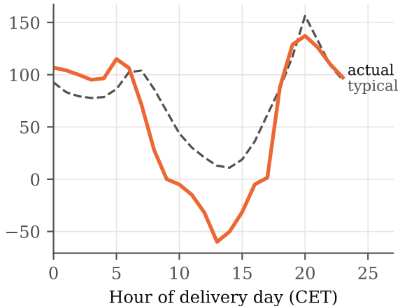
Sunniest day (11 Aug 2024): wind 15%, solar 37%
