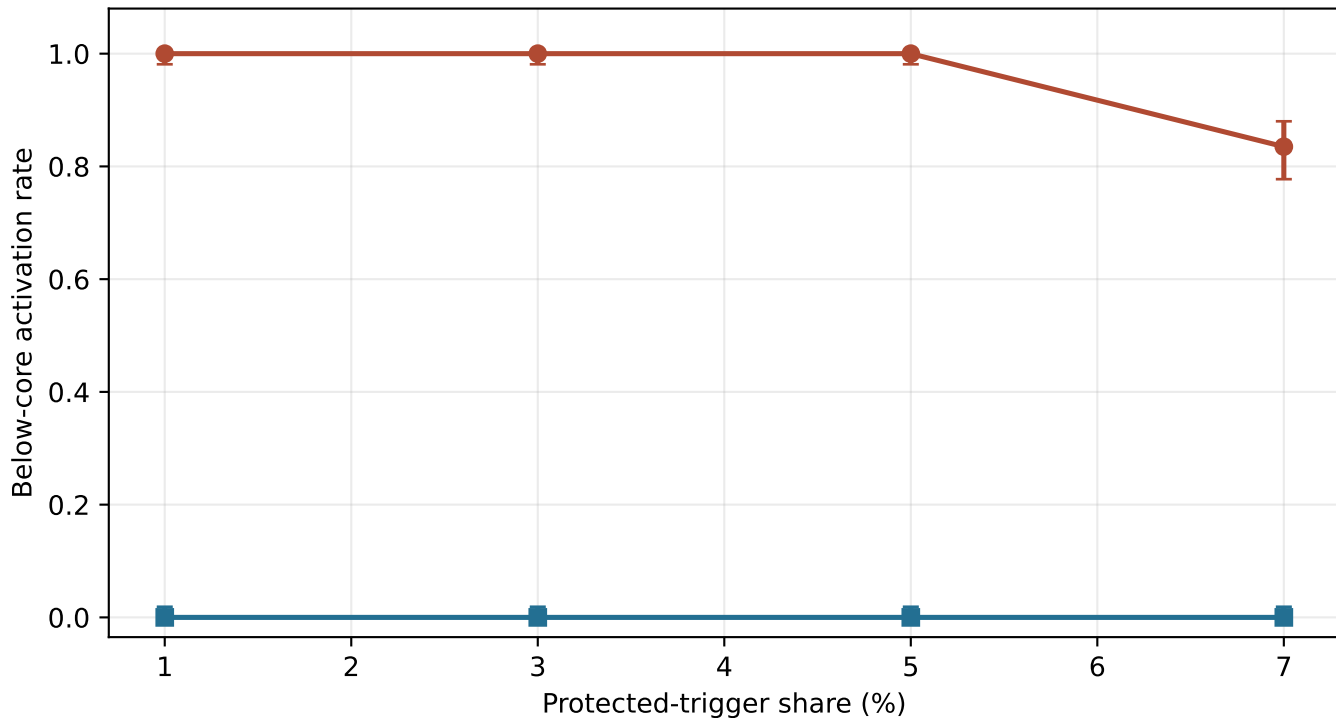
RQ2: core failure masked by aggregate success
