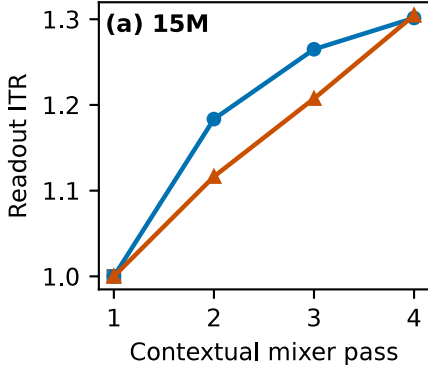
Cumulative directions
