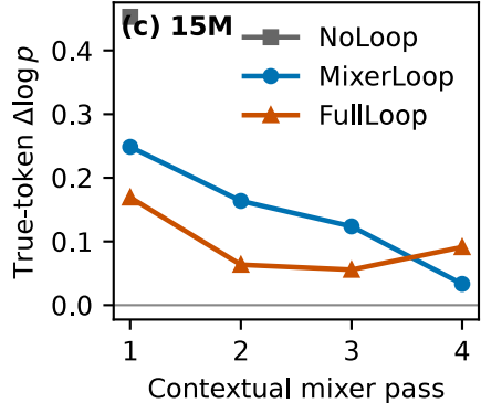
True-token contribution
