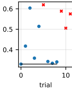
Task 2 specialists
