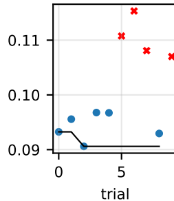
Task 4 cGAN
