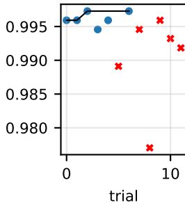
Task 2 classifier
