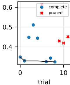
Task 1 (constrained)
