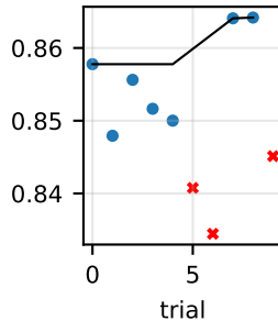
Task 3 MoE
