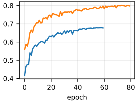
validation SSIM
