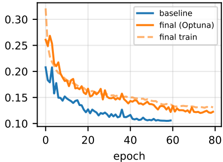
validation loss
