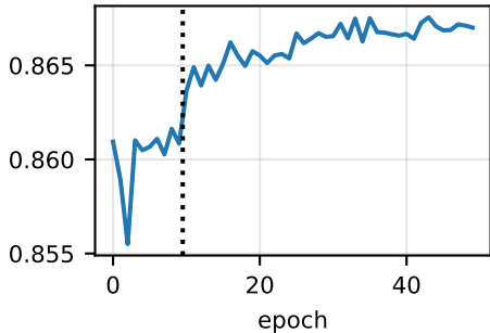
validation SSIM (warm-up | joint) mean routing weight on validation
