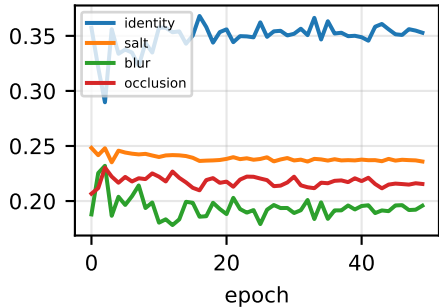
validation SSIM (warm-up | joint) mean routing weight on validation
