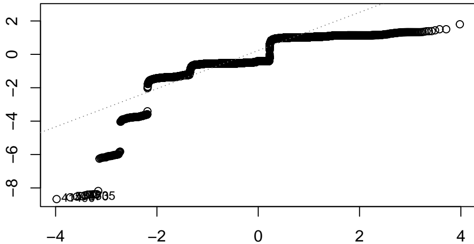
Q-Q Residuals
