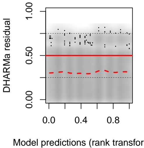
DHARMA residual vs. prediction
