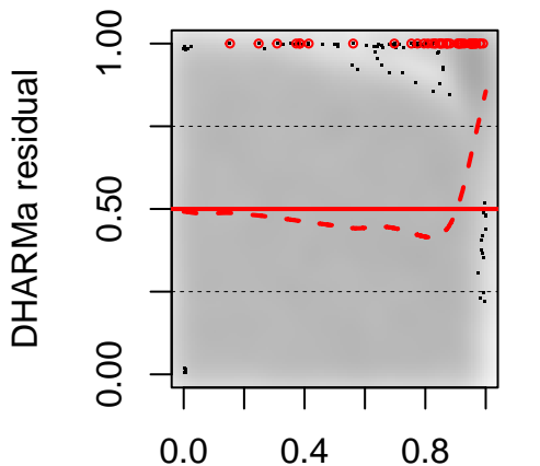
DHARMA residual vs. predic
