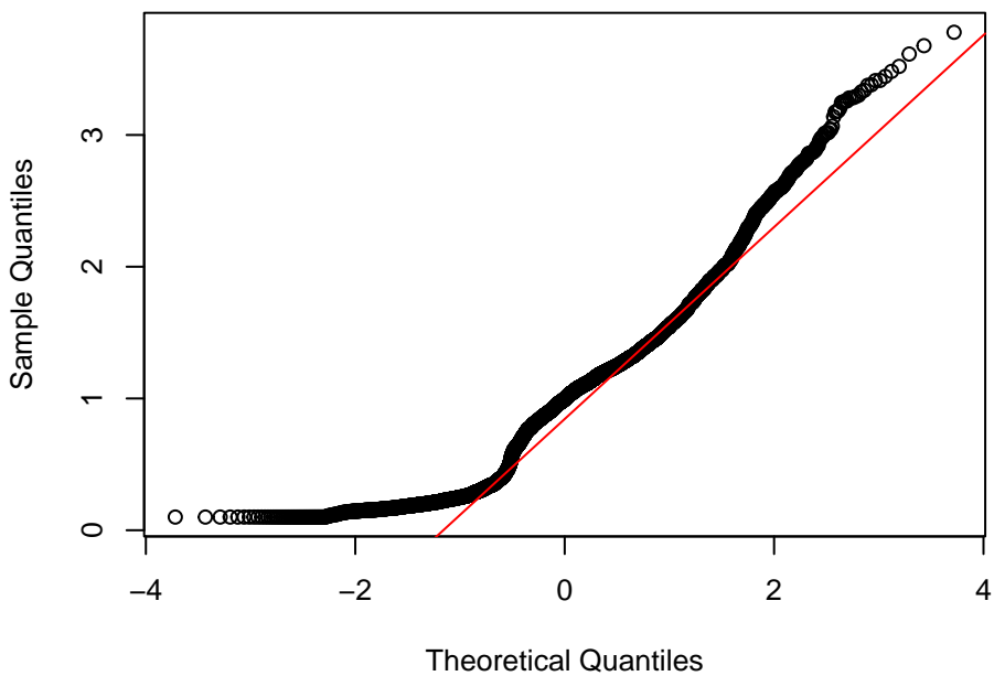
QQ: wtpumf vs Normal
