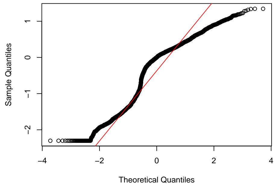
QQ: log(wtpumf) vs Normal
