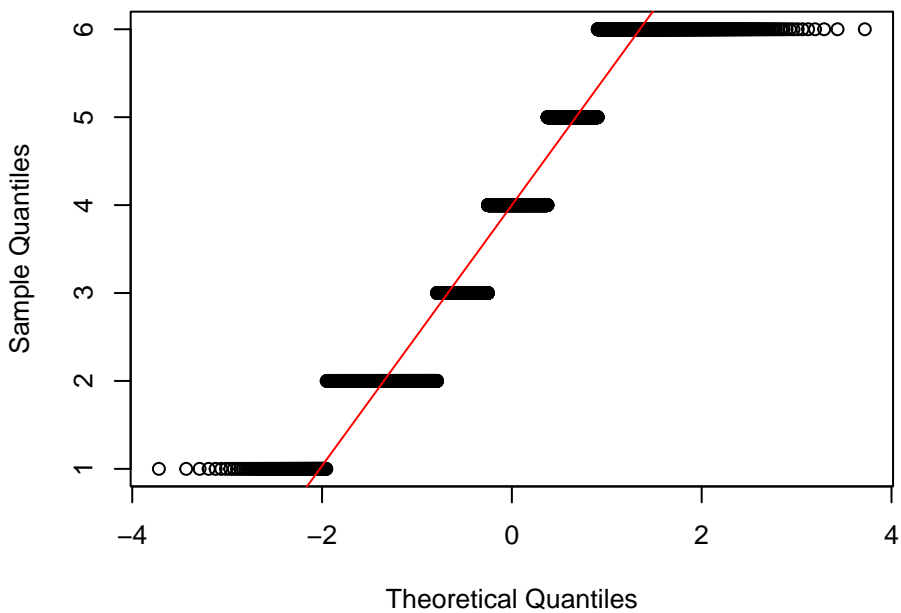
QQ: alc06 (ordinal code) vs Normal
