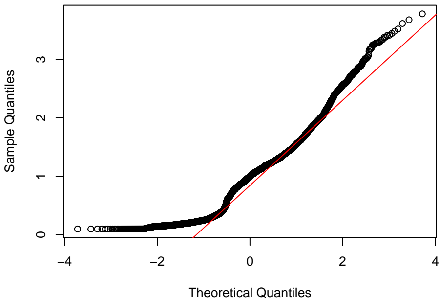
QQ: weight vs Normal
