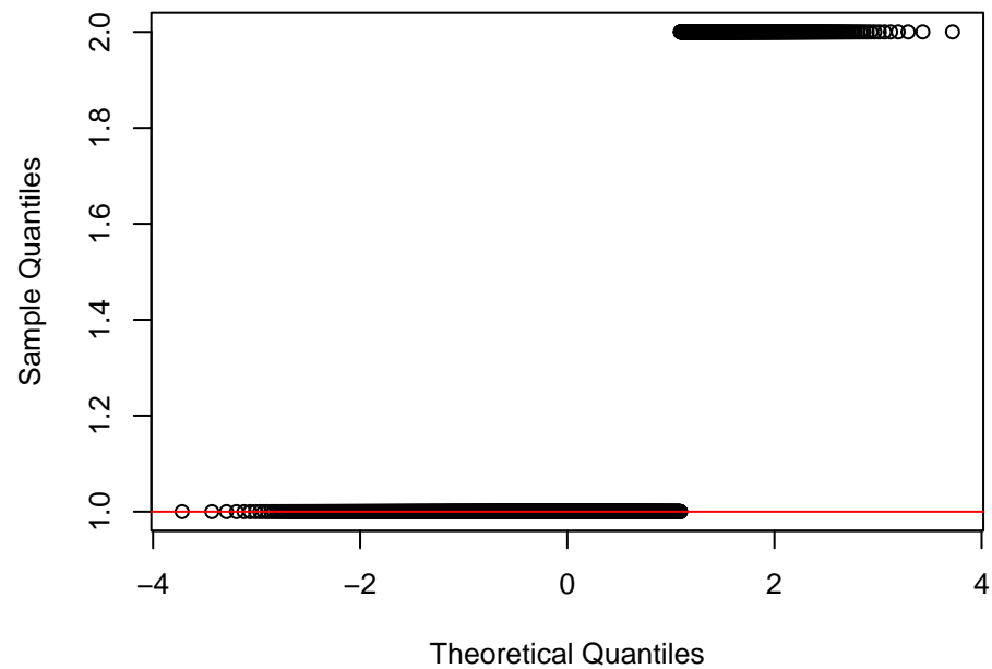
QQ: alc03 (ordinal code) vs Normal
