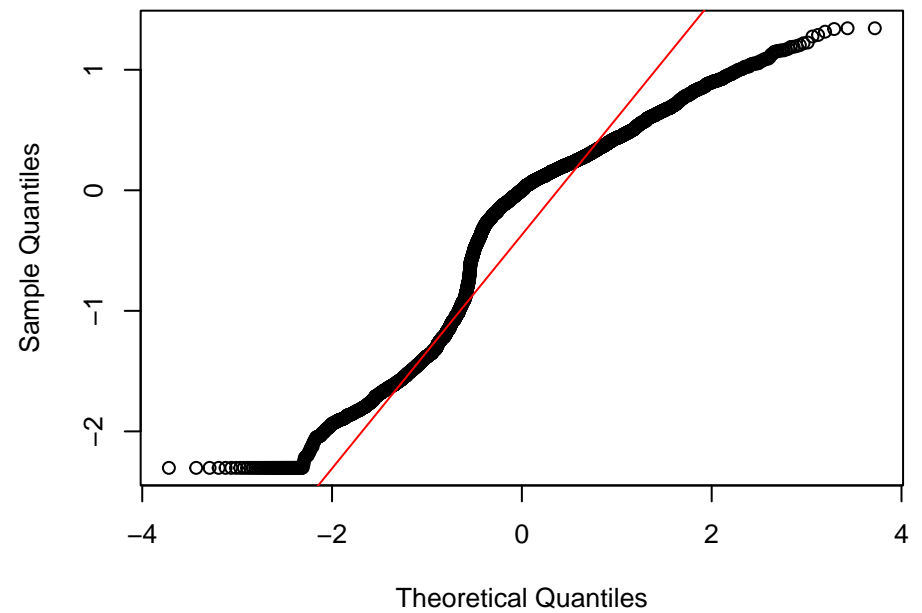
QQ: log(weight) vs Normal
