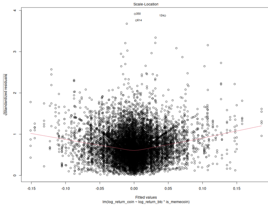
Figure 10: Scale-Location plot of fitted values vs. residuals.
