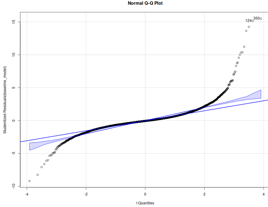
Figure 12: QQ plot of errors.
