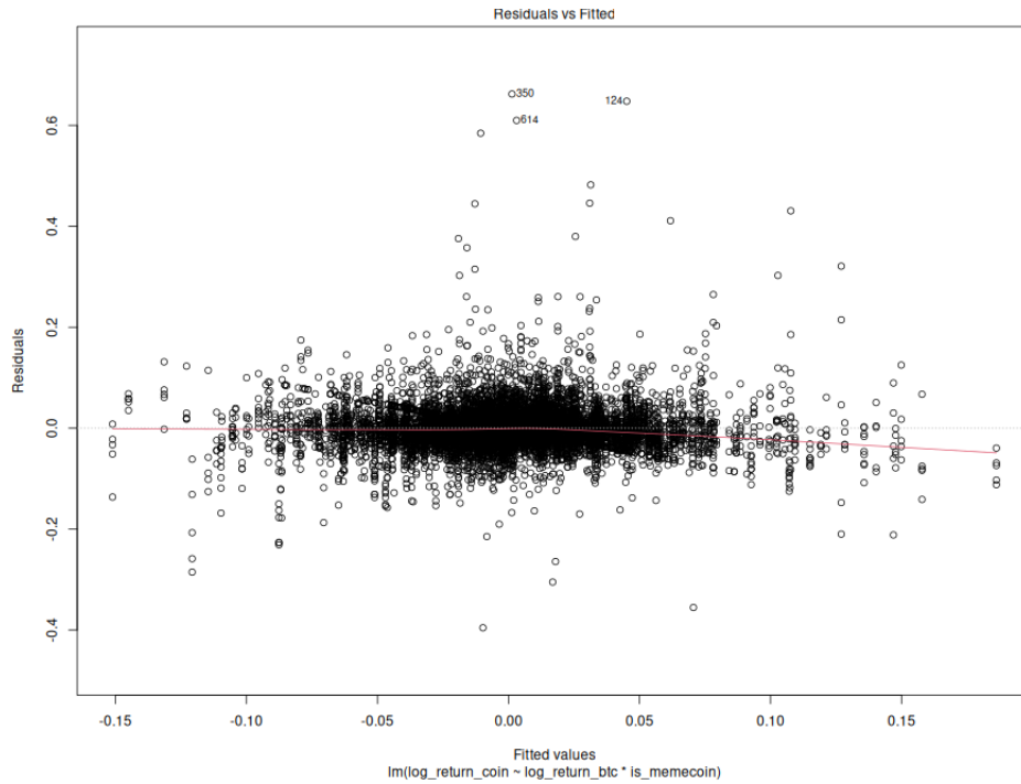
Figure 9: Residuals vs. Fitted Plot.
