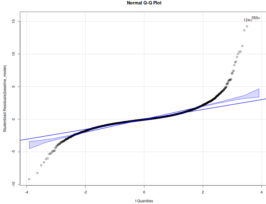
Figure 12: QQ plot of errors.
