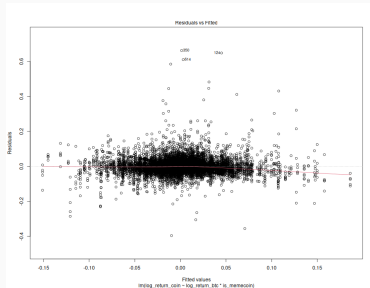
Figure 7: Left: Residuals vs. Fitted, Right: Scale-Location.
