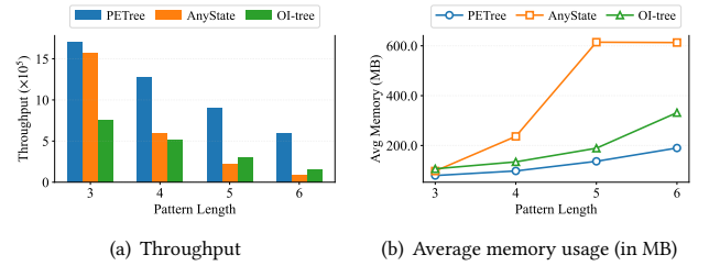
Figure 13: Evaluation on pattern length with a growing window
