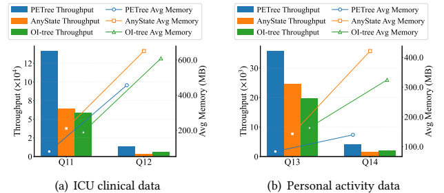
Figure 14: Performance on ICU and personal activity datasets
